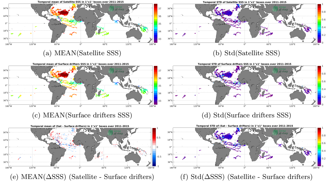
Figure 5: Temporal mean (left) and Std (right) of SSS from Aquarius SSS L3 CAP v5 - 7-Day running (JPL) (top), Surface drifters (middle), and of \Delta SSS (Satellite - Surface drifters). Only match-up pairs are used to generate these maps.
