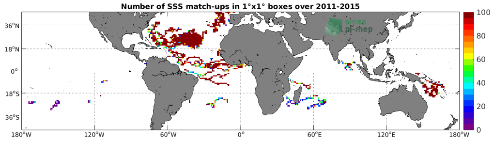
Figure 3: Number of SSS match-ups between Surface drifters SSS and the Aquarius SSS L3 CAP v5 - 7-Day running (JPL) SSS product for the Mid-Low Latitudes 45N-45S Pi-MEP region over 1°x1° boxes and for the full satellite product period.
