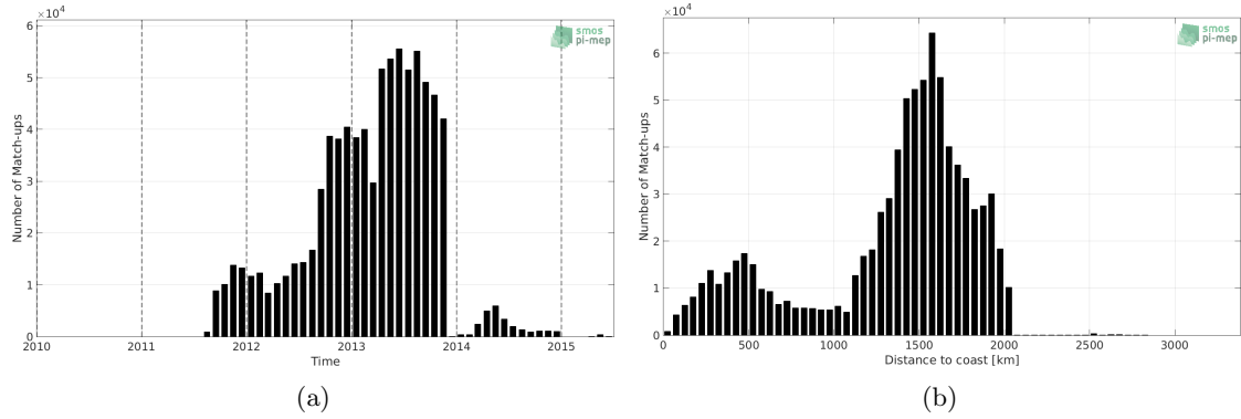
Figure 1: Number of match-ups between Surface drifters and Aquarius-L3-JPL-V5-7DAY-RUNNING SSS as a function of time (a) and as function of the distance to coast (b) over the Mid-Low Latitudes 45N-45S Pi-MEP region and for the full satellite product period.
