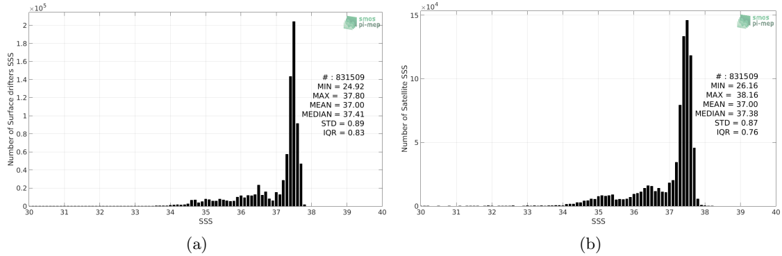
Figure 2: Histograms of SSS from Surface drifters (a) and Aquarius-L3-JPL-V5-7DAY-RUNNING (b) considering all match-up pairs per bins of 0.1 over the Mid-Low Latitudes 45N-45S Pi-MEP region and for the full satellite product period.
