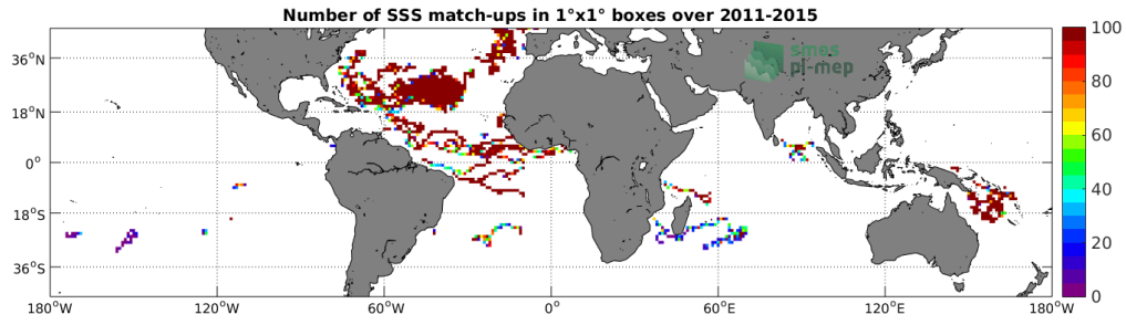
Figure 3: Number of SSS match-ups between Surface drifters SSS and the Aquarius-L3-JPL-V5-7DAY-RUNNING SSS product for the Mid-Low Latitudes 45N-45S Pi-MEP region over 1°x1° boxes and for the full satellite product period.
