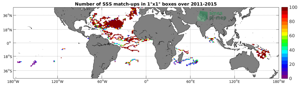
Figure 3: Number of SSS match-ups between Surface drifters SSS and the Aquarius-L3-JPL-V5-7DAY-RUNNING SSS product for the Mid-Low Latitudes 45N-45S Pi-MEP region over 1^\circ \times 1^\circ boxes and for the full satellite product period.
