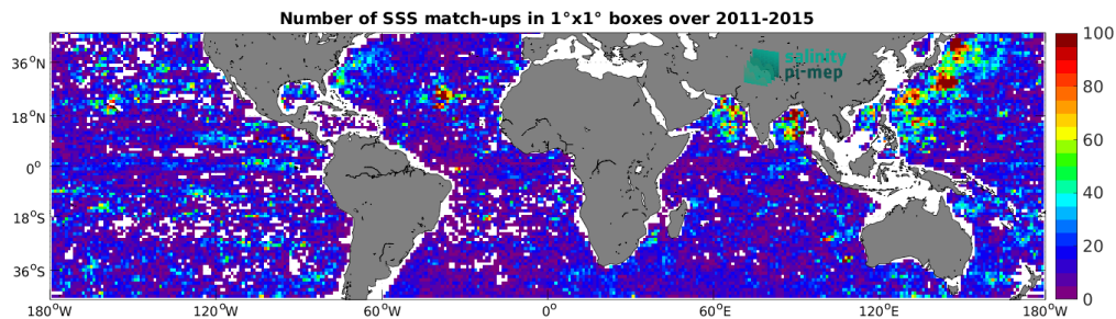
Figure 4: Number of SSS match-ups between Argo SSS and the Aquarius SSS L3 CAP v5 - 7-Day running (JPL) SSS product for the Mid-Low Latitudes 45N-45S Pi-MEP region over 1^\circ \times 1^\circ boxes and for the full satellite product period.
