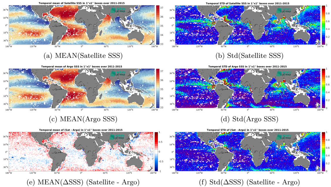
Figure 6: Temporal mean (left) and Std (right) of SSS from Aquarius SSS L3 CAP v5 - 7-Day running (JPL) (top), Argo (middle), and of \Delta SSS (Satellite - Argo). Only match-up pairs are used to generate these maps.
