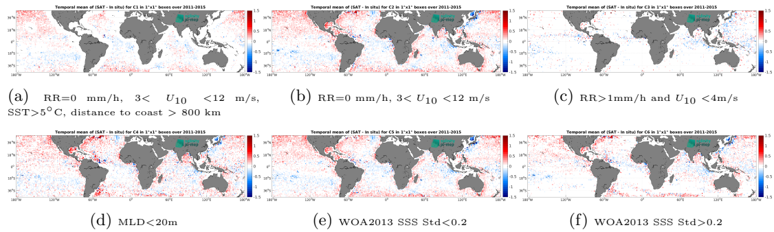
Figure 12: Temporal mean gridded over spatial boxes of size 1^\circ \times 1^\circ of \Delta SSS (Aquarius SSS L3 CAP v5 - 7-Day running (JPL) - Argo) for 6 different subdatasets corresponding to:RR=0 mm/h, 3 < U_{10} < 12 m/s, SST >5^\circ C, distance to coast > 800 km (a), RR=0 mm/h, 3 < U_{10} < 12 m/s (b), RR >1 mm/h and U_{10} < 4 m/s (c),MLD <20 m (d),WOA2013 SSS Std <0.2 (e),WOA2013 SSS Std >0.2 (f).
