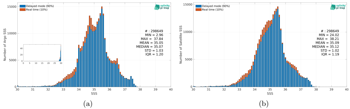
Figure 2: Histograms of SSS from Argo (a) and Aquarius SSS L3 CAP v5 - 7-Day running (JPL) (b) considering all match-up pairs per bins of 0.1 over the Mid-Low Latitudes 45N-45S Pi-MEP region and for the full satellite product period.
