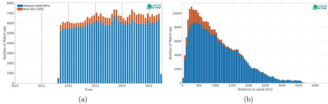
Figure 1: Number of match-ups between Argo and Aquarius SSS L3 CAP v5 - 7-Day running (JPL) SSS as a function of time (a) and as function of the distance to coast (b) over the Mid-Low Latitudes 45N-45S Pi-MEP region and for the full satellite product period.
