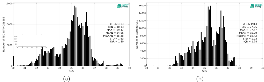
Figure 2: Histograms of SSS from TSG (SAMOS) (a) and Aquarius SSS L3 CAP v5 - Monthly (JPL) (b) considering all match-up pairs per bins of 0.1 over the Mid-Low Latitudes 45N-45S Pi-MEP region and for the full satellite product period.
