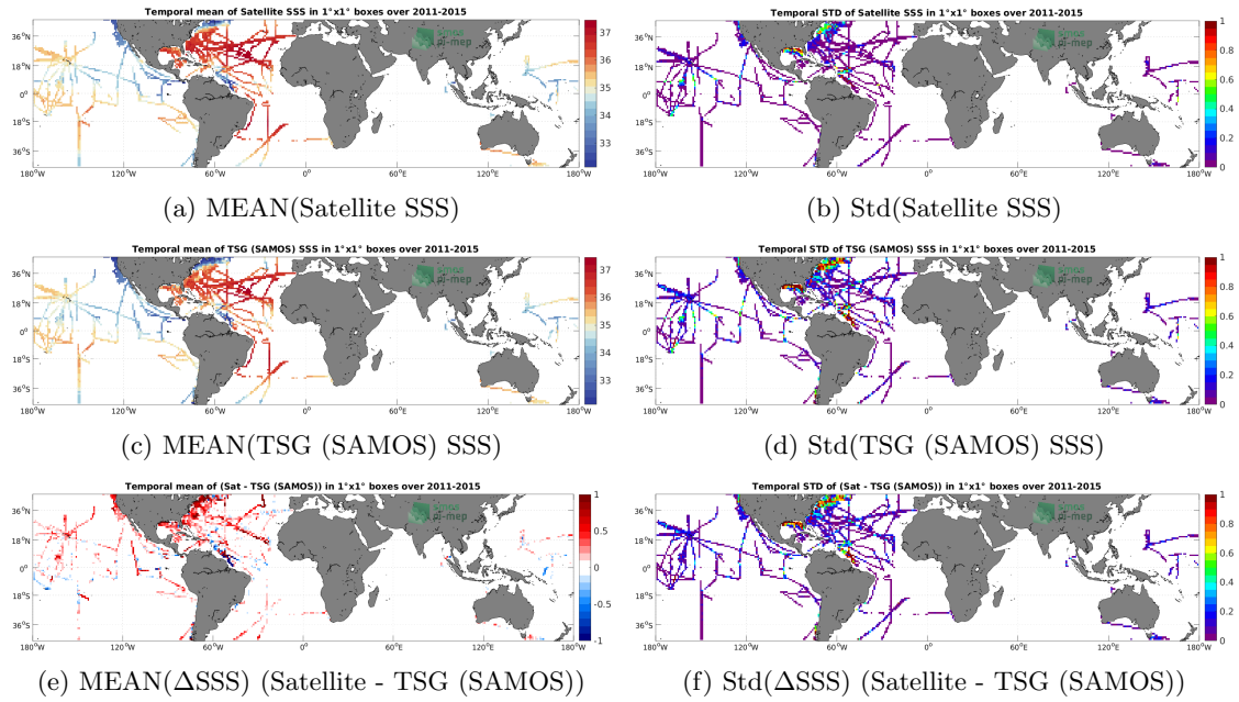
Figure 6: Temporal mean (left) and Std (right) of SSS from Aquarius SSS L3 CAP v5 - Monthly (JPL) (top), TSG (SAMOS) (middle), and of \Delta SSS (Satellite - TSG (SAMOS)). Only match-up pairs are used to generate these maps.
