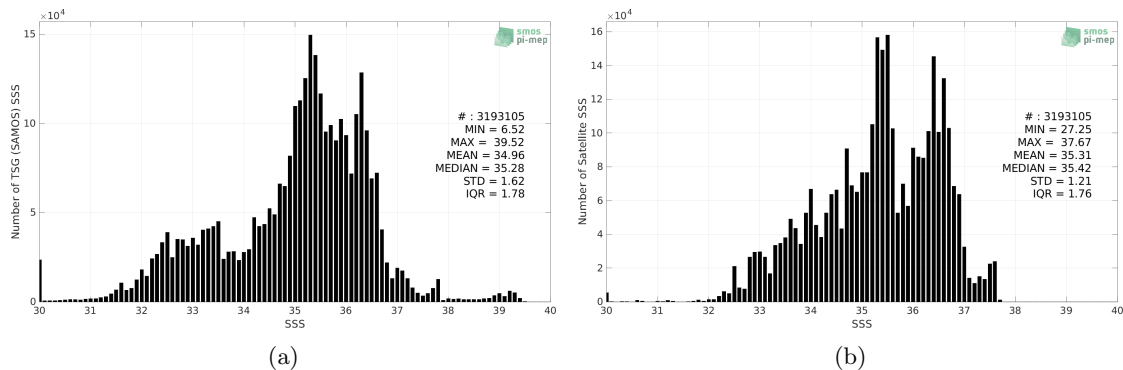
Figure 2: Histograms of SSS from TSG (SAMOS) (a) and Aquarius SSS L3 CAP v5 - Monthly (JPL) (b) considering all match-up pairs per bins of 0.1 over the Mid-Low Latitudes 45N-45S Pi-MEP region and for the full satellite product period.
