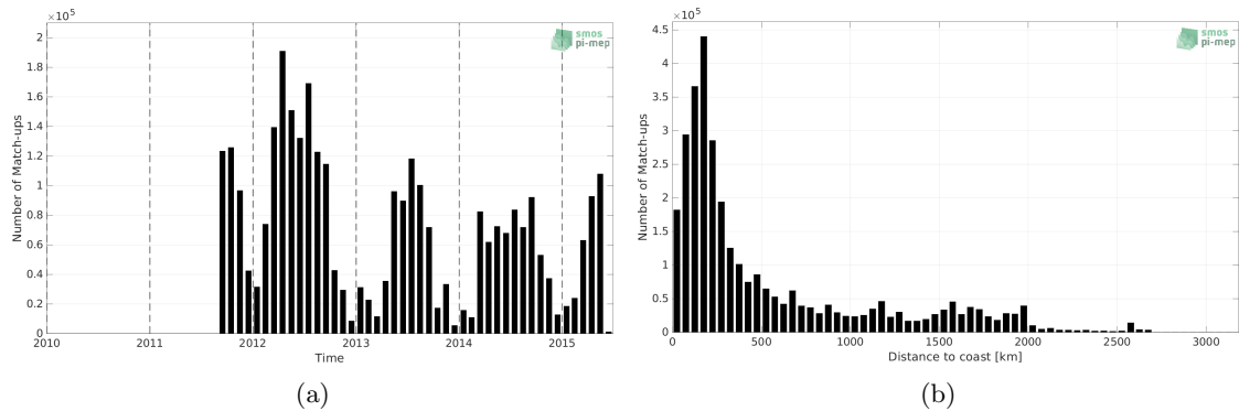
Figure 1: Number of match-ups between TSG (SAMOS) and Aquarius SSS L3 CAP v5 - Monthly (JPL) SSS as a function of time (a) and as function of the distance to coast (b) over the Mid-Low Latitudes 45N-45S Pi-MEP region and for the full satellite product period.
