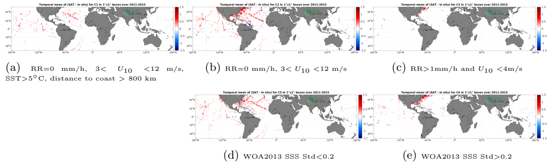
Figure 12: Temporal mean gridded over spatial boxes of size 1^\circ \times 1^\circ of \Delta SSS (Aquarius SSS L3 CAP v5 - Monthly (JPL) - TSG (SAMOS)) for 5 different subdatasets corresponding to:RR=0 mm/h, 3 < U_{10} < 12 m/s, SST >5^\circ C, distance to coast > 800 km (a), RR=0 mm/h, 3 < U_{10} < 12 m/s (b), RR >1 mm/h and U_{10} < 4 m/s (c), WOA2013 SSS Std <0.2 (d), WOA2013 SSS Std >0.2 (e).
