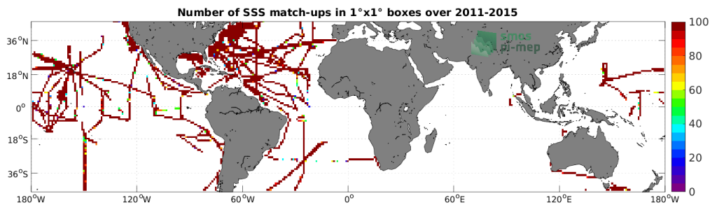
Figure 4: Number of SSS match-ups between TSG (SAMOS) SSS and the Aquarius SSS L3 CAP v5 - Monthly (JPL) SSS product for the Mid-Low Latitudes 45N-45S Pi-MEP region over 1^\circ \times 1^\circ boxes and for the full satellite product period.
