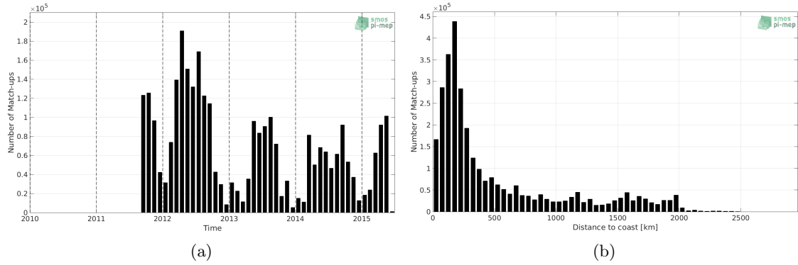
Figure 1: Number of match-ups between TSG-SAMOS and Aquarius-L3-JPL-V5-MONTHLY SSS as a function of time (a) and as function of the distance to coast (b) over the Mid-Low Latitudes 45N-45S Pi-MEP region and for the full satellite product period.
