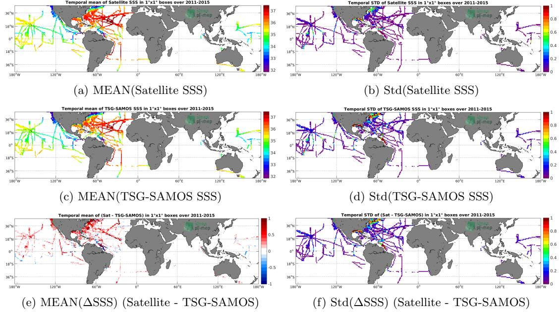
Figure 6: Temporal mean (left) and Std (right) of SSS from Aquarius-L3-JPL-V5-MONTHLY (top), TSG-SAMOS (middle), and of \Delta SSS (Satellite - TSG-SAMOS). Only match-up pairs are used to generate these maps.
