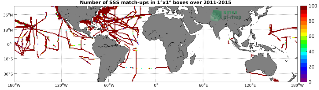
Figure 4: Number of SSS match-ups between TSG-SAMOS SSS and the Aquarius-L3-JPL-V5-MONTHLY SSS product for the Mid-Low Latitudes 45N-45S Pi-MEP region over 1^\circ \times 1^\circ boxes and for the full satellite product period.
