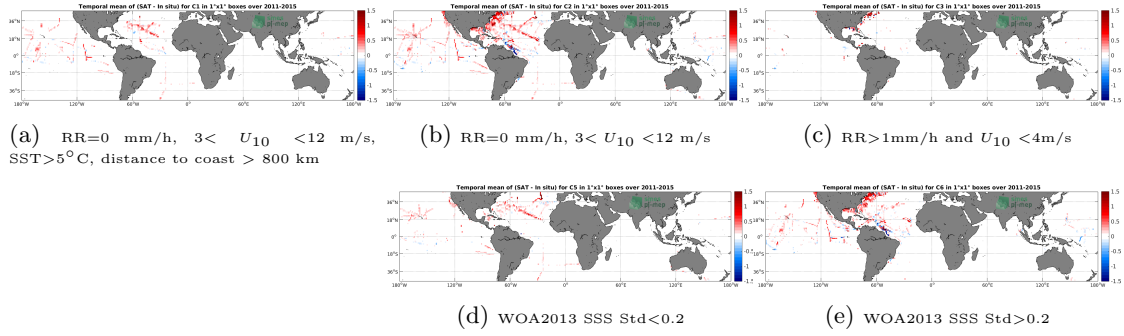
Figure 12: Temporal mean gridded over spatial boxes of size 1^\circ \times 1^\circ of \Delta SSS (Aquarius-L3-JPL-V5-MONTHLY - TSG-SAMOS) for 5 different subdatasets corresponding to: RR=0 mm/h, 3 < U_{10} < 12 m/s, SST > 5^\circ C , distance to coast > 800 km (a), RR=0 mm/h, 3 < U_{10} < 12 m/s (b), RR > 1 mm/h and U_{10} < 4 m/s (c), WOA2013 SSS Std < 0.2 (d), WOA2013 SSS Std > 0.2 (e).
