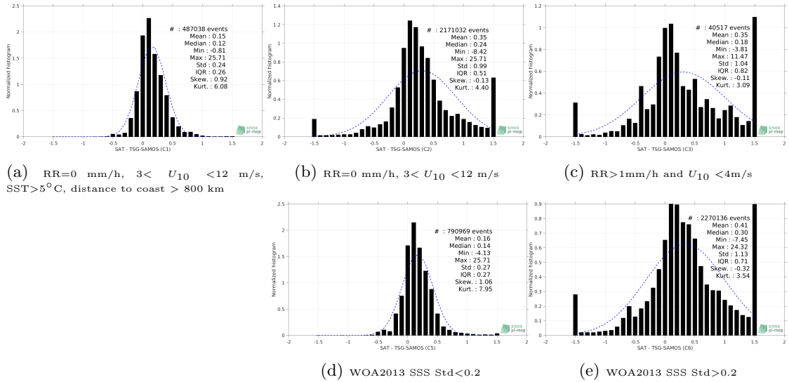
Figure 13: Normalized histogram of \Delta SSS (Aquarius-L3-JPL-V5-MONTHLY - TSG-SAMOS) for 5 different subdatasets corresponding to: RR=0 mm/h, 3 < U_{10} < 12 m/s, SST > 5^\circ C , distance to coast > 800 km (a), RR=0 mm/h, 3 < U_{10} < 12 m/s (b), RR > 1 mm/h and U_{10} < 4 m/s (c), WOA2013 SSS Std < 0.2 (d), WOA2013 SSS Std > 0.2 (e).
