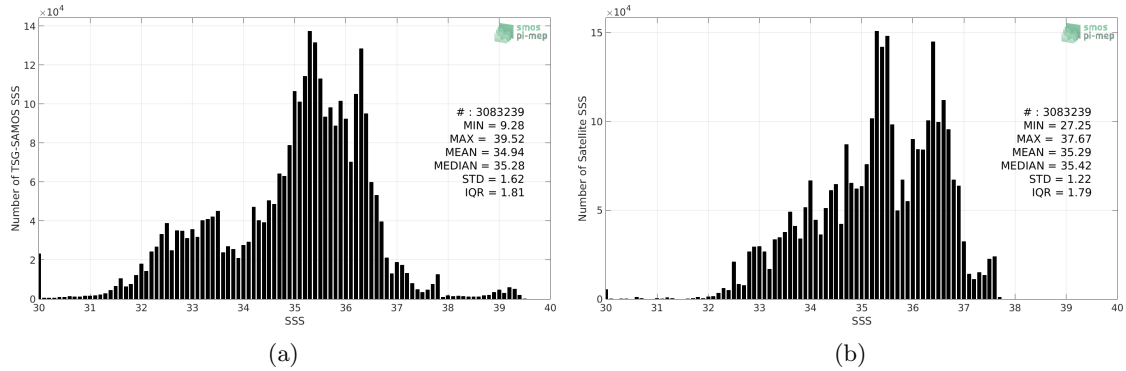
Figure 2: Histograms of SSS from TSG-SAMOS (a) and Aquarius-L3-JPL-V5-MONTHLY (b) considering all match-up pairs per bins of 0.1 over the Mid-Low Latitudes 45N-45S Pi-MEP region and for the full satellite product period.
