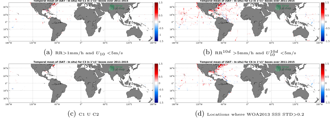
Figure 12: Temporal mean gridded over spatial boxes of size 1^\circ \times 1^\circ of \Delta SSS (Aquarius-L3-JPL-V5-MONTHLY - TSG-SAMOS) for 4 different subdatasets corresponding to: RR > 1mm/h and U_{10} < 5\text{m/s} (a), RR^{10d} > 5\text{mm/h} and U_{10}^{10d} < 5\text{m/s} (b), C1 U C2 (c), Locations where WOA2013 SSS STD > 0.2 (d).
