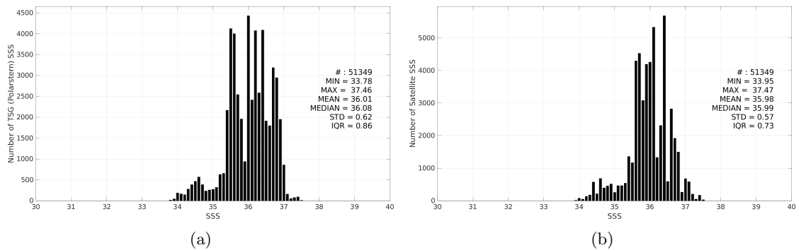
Figure 3: Histograms of SSS from TSG (Polarstern) (a) and Aquarius SSS L3 CAP v5 - Monthly (JPL) (b) considering all match-up pairs per bins of 0.1 over the Mid-Low Latitudes 45N-45S Pi-MEP region and for the full satellite product period.
