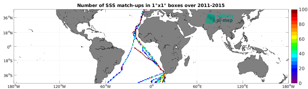
Figure 5: Number of SSS match-ups between TSG (Polarstern) SSS and the Aquarius SSS L3 CAP v5 - Monthly (JPL) SSS product for the Mid-Low Latitudes 45N-45S Pi-MEP region over 1^\circ \times 1^\circ boxes and for the full satellite product period.
