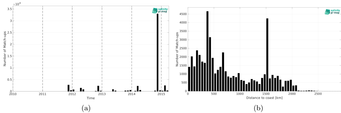
Figure 2: Number of match-ups between TSG (Polarstern) and Aquarius SSS L3 CAP v5 - Monthly (JPL) SSS as a function of time (a) and as function of the distance to coast (b) over the Mid-Low Latitudes 45N-45S Pi-MEP region and for the full satellite product period.
