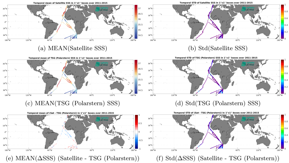
Figure 7: Temporal mean (left) and Std (right) of SSS from Aquarius SSS L3 CAP v5 - Monthly (JPL) (top), TSG (Polarstern) (middle), and of \Delta SSS (Satellite - TSG (Polarstern)). Only match-up pairs are used to generate these maps.
