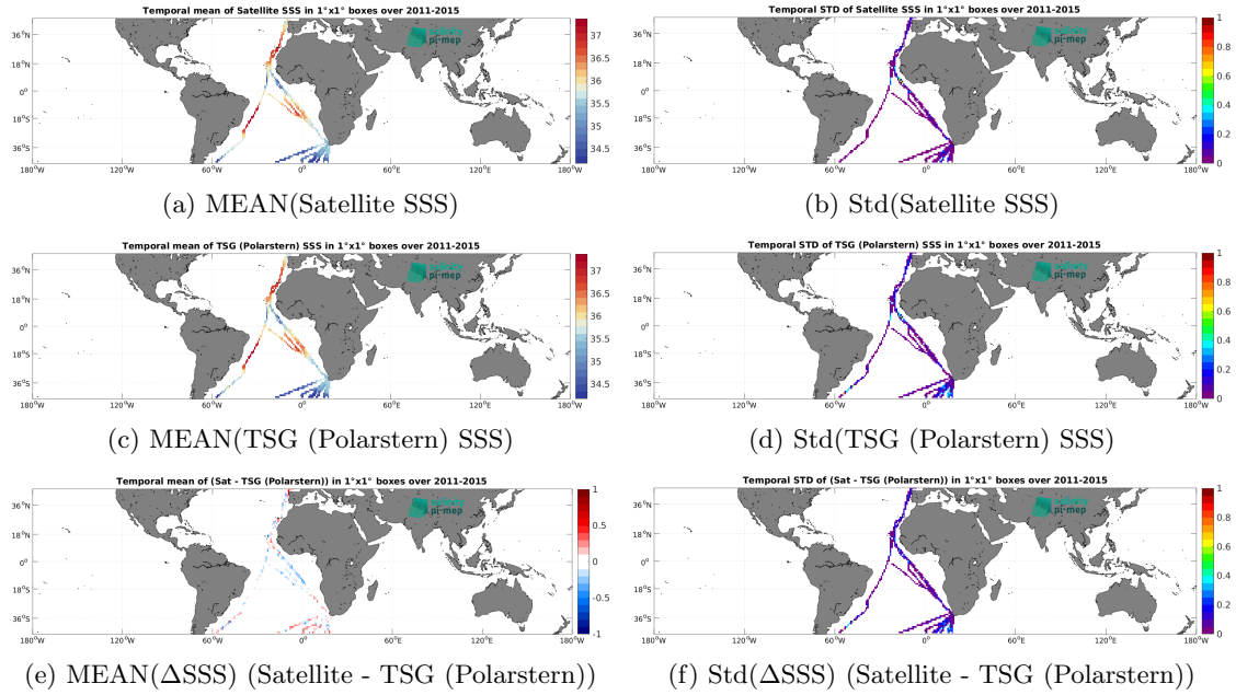
Figure 6: Temporal mean (left) and Std (right) of SSS from Aquarius SSS L3 CAP v5 - Monthly (JPL) (top), TSG (Polarstern) (middle), and of \Delta SSS (Satellite - TSG (Polarstern)). Only match-up pairs are used to generate these maps.
