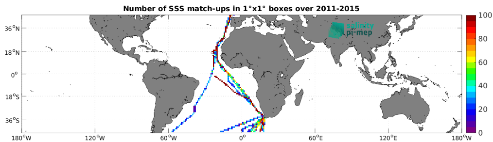
Figure 4: Number of SSS match-ups between TSG (Polarstern) SSS and the Aquarius SSS L3 CAP v5 - Monthly (JPL) SSS product for the Mid-Low Latitudes 45N-45S Pi-MEP region over 1^\circ \times 1^\circ boxes and for the full satellite product period.
