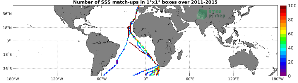
Figure 4: Number of SSS match-ups between TSG (Polarstern) SSS and the Aquarius SSS L3 CAP v5 - Monthly (JPL) SSS product for the Mid-Low Latitudes 45N-45S Pi-MEP region over 1°x1° boxes and for the full satellite product period.
