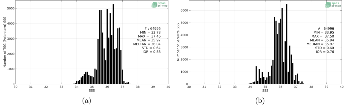
Figure 2: Histograms of SSS from TSG (Polarstern) (a) and Aquarius SSS L3 CAP v5 - Monthly (JPL) (b) considering all match-up pairs per bins of 0.1 over the Mid-Low Latitudes 45N-45S Pi-MEP region and for the full satellite product period.
