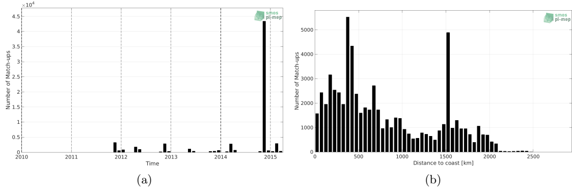
Figure 1: Number of match-ups between TSG (Polarstern) and Aquarius SSS L3 CAP v5 - Monthly (JPL) SSS as a function of time (a) and as function of the distance to coast (b) over the Mid-Low Latitudes 45N-45S Pi-MEP region and for the full satellite product period.
