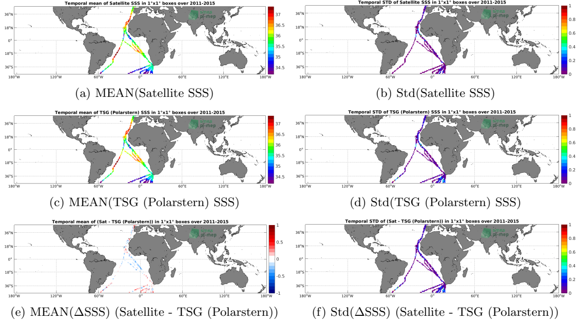
Figure 6: Temporal mean (left) and Std (right) of SSS from Aquarius SSS L3 CAP v5 - Monthly (JPL) (top), TSG (Polarstern) (middle), and of \Delta SSS (Satellite - TSG (Polarstern)). Only match-up pairs are used to generate these maps.
