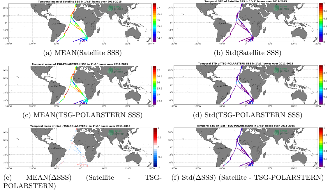
Figure 6: Temporal mean (left) and Std (right) of SSS from Aquarius-L3-JPL-V5-MONTHLY (top), TSG-POLARSTERN (middle), and of \Delta SSS (Satellite - TSG-POLARSTERN). Only match-up pairs are used to generate these maps.
