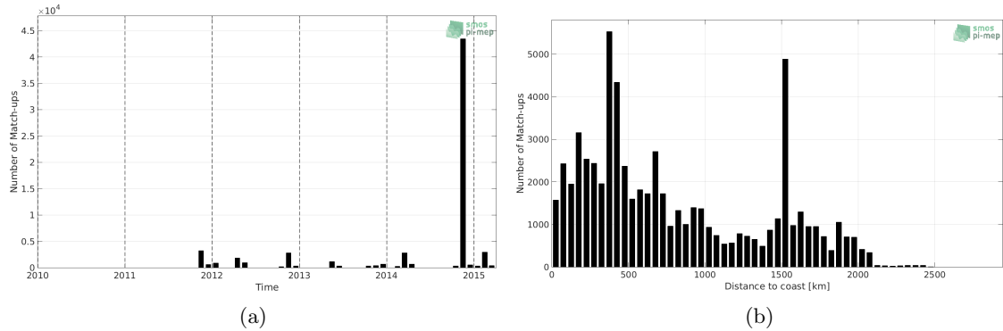
Figure 1: Number of match-ups between TSG-POLARSTERN and Aquarius-L3-JPL-V5-MONTHLY SSS as a function of time (a) and as function of the distance to coast (b) over the Mid-Low Latitudes 45N-45S Pi-MEP region and for the full satellite product period.
