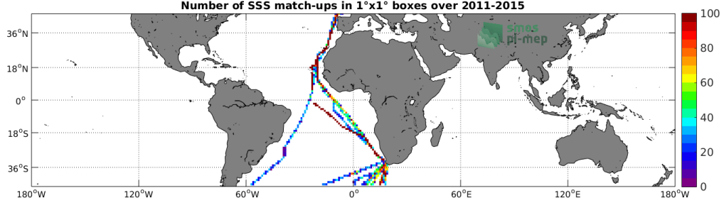
Figure 4: Number of SSS match-ups between TSG-POLARSTERN SSS and the Aquarius-L3-JPL-V5-MONTHLY SSS product for the Mid-Low Latitudes 45N-45S Pi-MEP region over 1^\circ \times 1^\circ boxes and for the full satellite product period.
