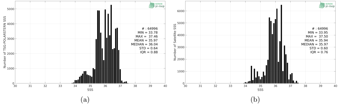
Figure 2: Histograms of SSS from TSG-POLARSTERN (a) and Aquarius-L3-JPL-V5-MONTHLY (b) considering all match-up pairs per bins of 0.1 over the Mid-Low Latitudes 45N-45S Pi-MEP region and for the full satellite product period.
