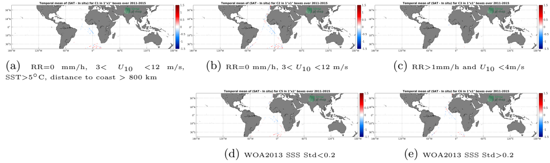
Figure 12: Temporal mean gridded over spatial boxes of size 1^\circ \times 1^\circ of \Delta SSS (Aquarius-L3-JPL-V5-MONTHLY - TSG-POLARSTERN) for 5 different subdatasets corresponding to: RR=0 mm/h, 3 < U_{10} < 12 m/s, SST > 5^\circ C , distance to coast > 800 km (a), RR=0 mm/h, 3 < U_{10} < 12 m/s (b), RR > 1 mm/h and U_{10} < 4 m/s (c), WOA2013 SSS Std < 0.2 (d), WOA2013 SSS Std > 0.2 (e).
