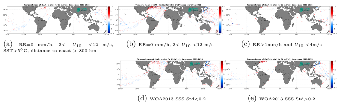
Figure 14: Temporal mean gridded over spatial boxes of size 1^\circ \times 1^\circ of \Delta\text{SSS} (Aquarius SSS L3 CAP v5 - Monthly (JPL) - TSG (LEGOS-DM)) for 5 different subdatasets corresponding to:RR=0 mm/h, 3 < U_{10} < 12 m/s, SST > 5°C, distance to coast > 800 km (a), RR=0 mm/h, 3 < U_{10} < 12 m/s (b), RR > 1mm/h and U_{10} < 4 m/s (c), WOA2013 SSS Std < 0.2 (d), WOA2013 SSS Std > 0.2 (e).
