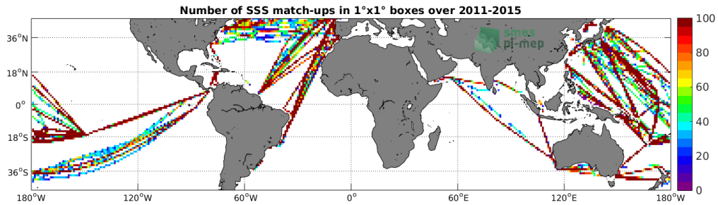
Figure 4: Number of SSS match-ups between TSG-LEGOS-DM SSS and the Aquarius-L3-JPL-V5-MONTHLY SSS product for the Mid-Low Latitudes 45N-45S Pi-MEP region over 1^\circ \times 1^\circ boxes and for the full satellite product period.
