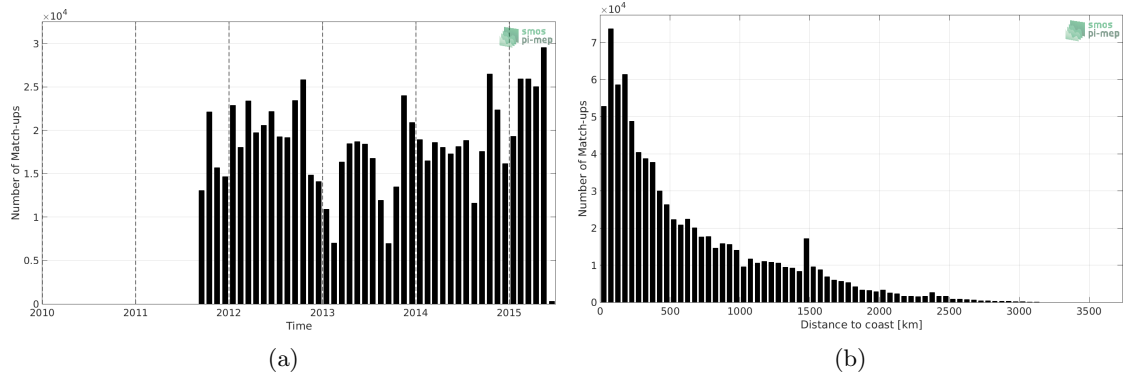
Figure 1: Number of match-ups between TSG-LEGOS-DM and Aquarius-L3-JPL-V5-MONTHLY SSS as a function of time (a) and as function of the distance to coast (b) over the Mid-Low Latitudes 45N-45S Pi-MEP region and for the full satellite product period.
