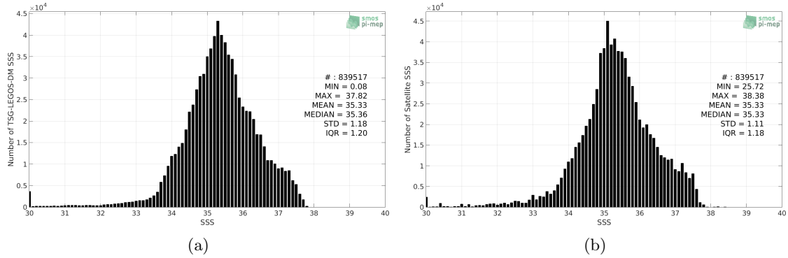
Figure 2: Histograms of SSS from TSG-LEGOS-DM (a) and Aquarius-L3-JPL-V5-MONTHLY (b) considering all match-up pairs per bins of 0.1 over the Mid-Low Latitudes 45N-45S Pi-MEP region and for the full satellite product period.
