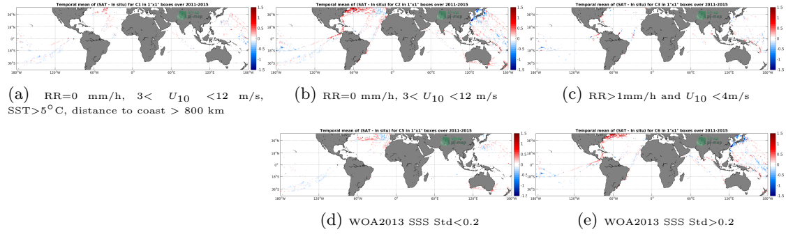
Figure 12: Temporal mean gridded over spatial boxes of size 1^\circ \times 1^\circ of \Delta SSS (Aquarius-L3-JPL-V5-MONTHLY - TSG-LEGOS-DM) for 5 different subdatasets corresponding to:RR=0 mm/h, 3 < U_{10} < 12 m/s, SST >5^\circ\text{C} , distance to coast > 800 km (a), RR=0 mm/h, 3 < U_{10} < 12 m/s (b), RR >1 mm/h and U_{10} < 4 m/s (c), WOA2013 SSS Std <0.2 (d), WOA2013 SSS Std >0.2 (e).
