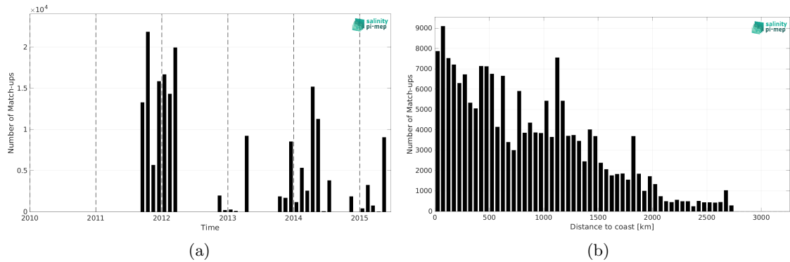
Figure 2: Number of match-ups between TSG (GOSUD-Sailing-ship) and Aquarius SSS L3 CAP v5 - Monthly (JPL) SSS as a function of time (a) and as function of the distance to coast (b) over the Mid-Low Latitudes 45N-45S Pi-MEP region and for the full satellite product period.
