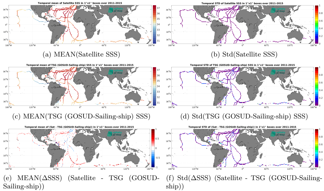
Figure 7: Temporal mean (left) and Std (right) of SSS from Aquarius SSS L3 CAP v5 - Monthly (JPL) (top), TSG (GOSUD-Sailing-ship) (middle), and of \Delta SSS (Satellite - TSG (GOSUD-Sailing-ship)). Only match-up pairs are used to generate these maps.
