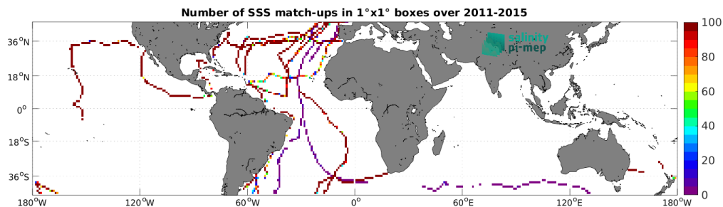
Figure 5: Number of SSS match-ups between TSG (GOSUD-Sailing-ship) SSS and the Aquarius SSS L3 CAP v5 - Monthly (JPL) SSS product for the Mid-Low Latitudes 45N-45S Pi-MEP region over 1^\circ \times 1^\circ boxes and for the full satellite product period.
