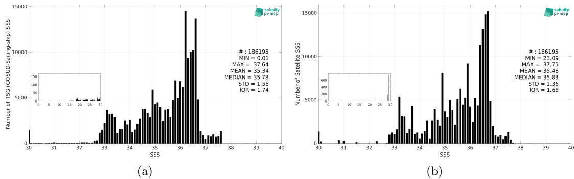
Figure 3: Histograms of SSS from TSG (GOSUD-Sailing-ship) (a) and Aquarius SSS L3 CAP v5 - Monthly (JPL) (b) considering all match-up pairs per bins of 0.1 over the Mid-Low Latitudes 45N-45S Pi-MEP region and for the full satellite product period.
