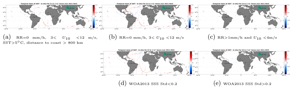
Figure 14: Temporal mean gridded over spatial boxes of size 1^\circ \times 1^\circ of \Delta SSS (Aquarius SSS L3 CAP v5 - Monthly (JPL) - TSG (GOSUD-Sailing-ship)) for 5 different subdatasets corresponding to:RR=0 mm/h, 3 < U_{10} < 12 m/s, SST>5°C, distance to coast > 800 km (a), RR=0 mm/h, 3 < U_{10} < 12 m/s (b), RR>1mm/h and U_{10} < 4 m/s (c), WOA2013 SSS Std<0.2 (d), WOA2013 SSS Std>0.2 (e).
