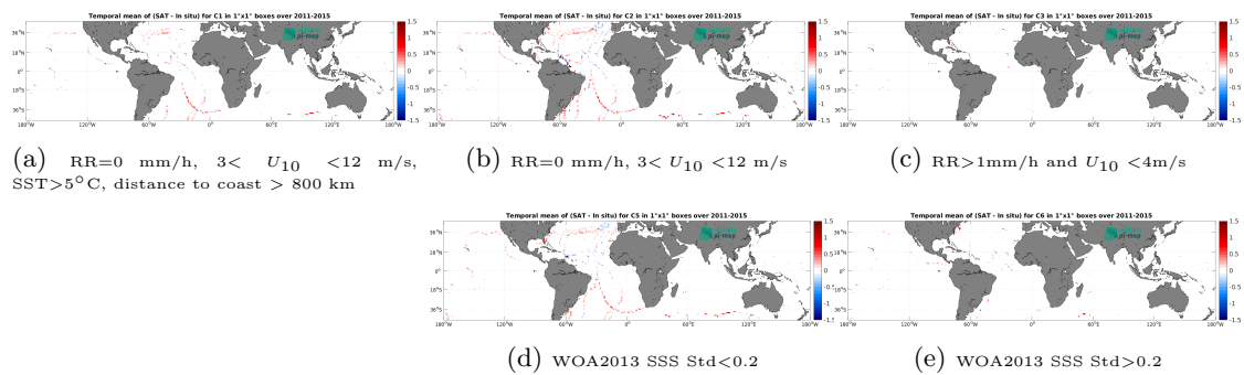
Figure 14: Temporal mean gridded over spatial boxes of size 1^\circ \times 1^\circ of \Delta\text{SSS} (Aquarius SSS L3 CAP v5 - Monthly (JPL) - TSG (GOSUD-Sailing-ship)) for 5 different subdatasets corresponding to: RR=0 mm/h, 3 < U_{10} < 12 m/s, SST > 5°C, distance to coast > 800 km (a), RR=0 mm/h, 3 < U_{10} < 12 m/s (b), RR > 1mm/h and U_{10} < 4 m/s (c), WOA2013 SSS Std < 0.2 (d), WOA2013 SSS Std > 0.2 (e).
