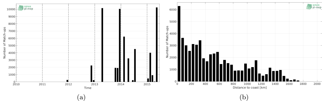
Figure 1: Number of match-ups between TSG-GOSUD-Sailing-ship and Aquarius-L3-JPL-V5-MONTHLY SSS as a function of time (a) and as function of the distance to coast (b) over the Mid-Low Latitudes 45N-45S Pi-MEP region and for the full satellite product period.
