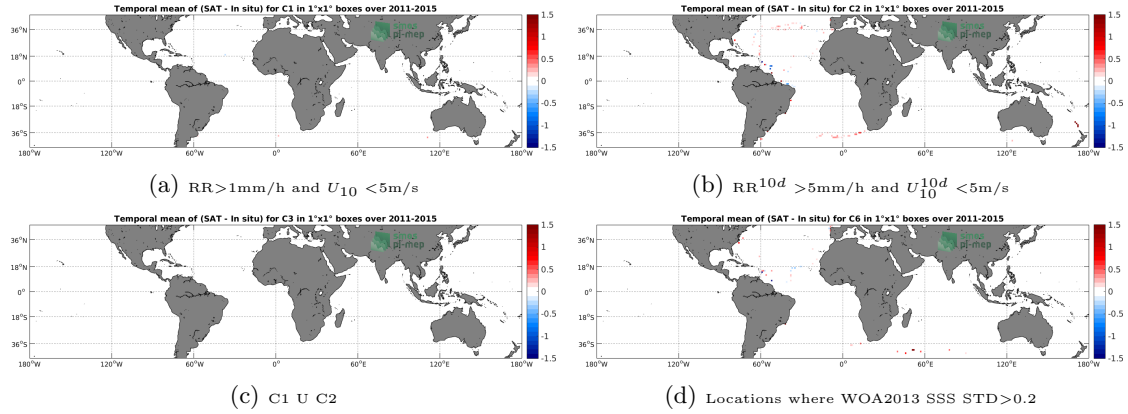
Figure 12: Temporal mean gridded over spatial boxes of size 1^\circ \times 1^\circ of \Delta SSS (Aquarius-L3-JPL-V5-MONTHLY - TSG-GOSUD-Sailing-ship) for 4 different subdatasets corresponding to: RR > 1\text{mm/h} and U_{10} < 5\text{m/s} (a), RR^{10d} > 5\text{mm/h} and U_{10}^{10d} < 5\text{m/s} (b), C1 U C2 (c), Locations where WOA2013 SSS STD > 0.2 (d).
