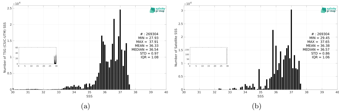
Figure 3: Histograms of SSS from TSG (CSIC-UTM) (a) and Aquarius SSS L3 CAP v5 - Monthly (JPL) (b) considering all match-up pairs per bins of 0.1 over the Mid-Low Latitudes 45N-45S Pi-MEP region and for the full satellite product period.
