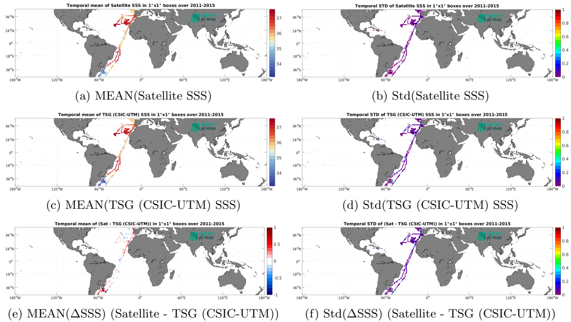
Figure 7: Temporal mean (left) and Std (right) of SSS from Aquarius SSS L3 CAP v5 - Monthly (JPL) (top), TSG (CSIC-UTM) (middle), and of \Delta SSS (Satellite - TSG (CSIC-UTM)). Only match-up pairs are used to generate these maps.
