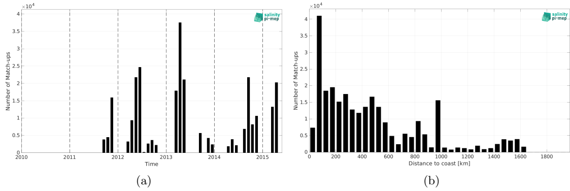
Figure 2: Number of match-ups between TSG (CSIC-UTM) and Aquarius SSS L3 CAP v5 - Monthly (JPL) SSS as a function of time (a) and as function of the distance to coast (b) over the Mid-Low Latitudes 45N-45S Pi-MEP region and for the full satellite product period.
