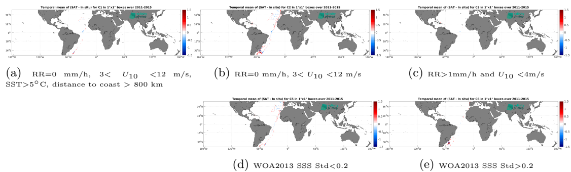
Figure 14: Temporal mean gridded over spatial boxes of size 1^\circ \times 1^\circ of \Delta\text{SSS} (Aquarius SSS L3 CAP v5 - Monthly (JPL) - TSG (CSIC-UTM)) for 5 different subdatasets corresponding to: RR=0 mm/h, 3 < U_{10} < 12 m/s, SST > 5°C, distance to coast > 800 km (a), RR=0 mm/h, 3 < U_{10} < 12 m/s (b), RR > 1mm/h and U_{10} < 4 m/s (c), WOA2013 SSS Std < 0.2 (d), WOA2013 SSS Std > 0.2 (e).
