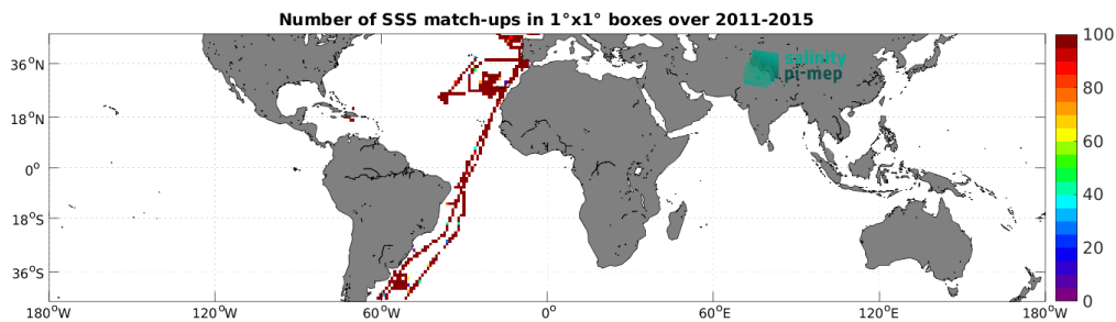
Figure 5: Number of SSS match-ups between TSG (CSIC-UTM) SSS and the Aquarius SSS L3 CAP v5 - Monthly (JPL) SSS product for the Mid-Low Latitudes 45N-45S Pi-MEP region over 1^\circ \times 1^\circ boxes and for the full satellite product period.
