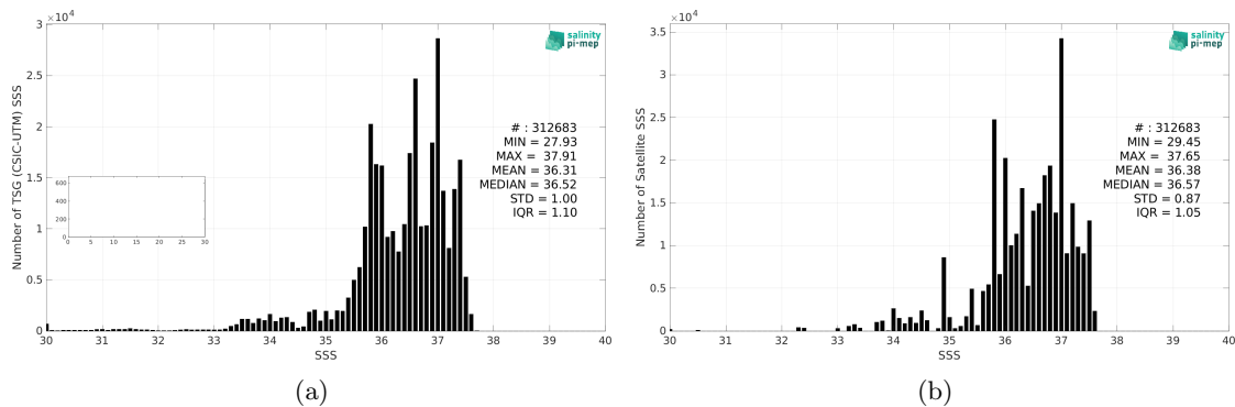
Figure 2: Histograms of SSS from TSG (CSIC-UTM) (a) and Aquarius SSS L3 CAP v5 - Monthly (JPL) (b) considering all match-up pairs per bins of 0.1 over the Mid-Low Latitudes 45N-45S Pi-MEP region and for the full satellite product period.
