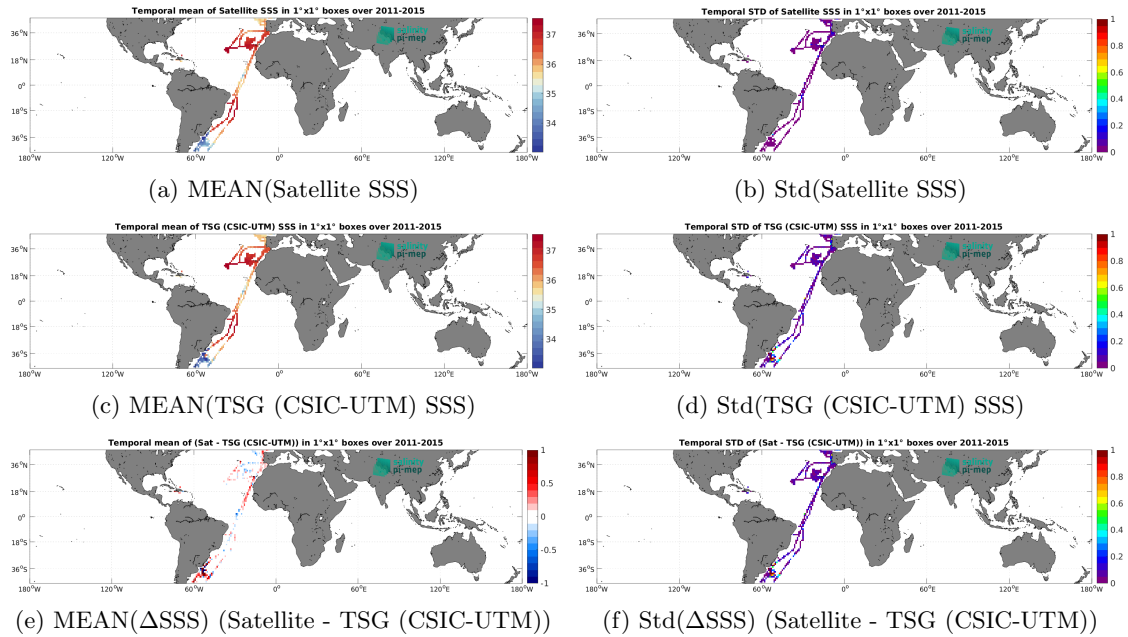
Figure 6: Temporal mean (left) and Std (right) of SSS from Aquarius SSS L3 CAP v5 - Monthly (JPL) (top), TSG (CSIC-UTM) (middle), and of \Delta SSS (Satellite - TSG (CSIC-UTM)). Only match-up pairs are used to generate these maps.
