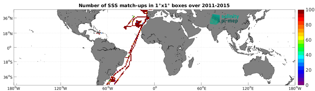
Figure 4: Number of SSS match-ups between TSG (CSIC-UTM) SSS and the Aquarius SSS L3 CAP v5 - Monthly (JPL) SSS product for the Mid-Low Latitudes 45N-45S Pi-MEP region over 1^\circ \times 1^\circ boxes and for the full satellite product period.
