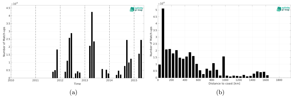
Figure 1: Number of match-ups between TSG (CSIC-UTM) and Aquarius SSS L3 CAP v5 - Monthly (JPL) SSS as a function of time (a) and as function of the distance to coast (b) over the Mid-Low Latitudes 45N-45S Pi-MEP region and for the full satellite product period.
