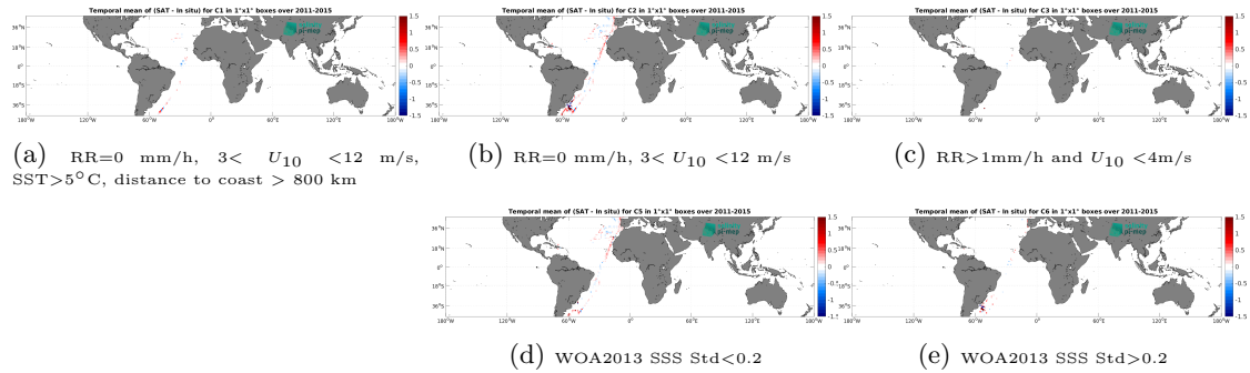
Figure 12: Temporal mean gridded over spatial boxes of size 1^\circ \times 1^\circ of \Delta SSS (Aquarius SSS L3 CAP v5 - Monthly (JPL) - TSG (CSIC-UTM)) for 5 different subdatasets corresponding to:RR=0 mm/h, 3 < U_{10} < 12 m/s, SST>5°C, distance to coast > 800 km (a), RR=0 mm/h, 3 < U_{10} < 12 m/s (b), RR>1mm/h and U_{10} < 4 m/s (c), WOA2013 SSS Std<0.2 (d), WOA2013 SSS Std>0.2 (e).
