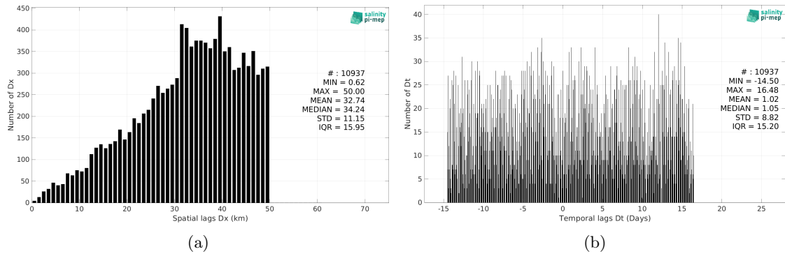
Figure 6: Histograms of the spatial (a) and temporal (b) lags between the location/time of the Marine mammals measurement and the date of the corresponding Aquarius SSS L3 CAP v5 - Monthly (JPL) SSS pixel.
