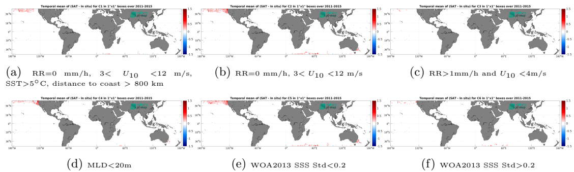
Figure 14: Temporal mean gridded over spatial boxes of size 1^\circ \times 1^\circ of \Delta\text{SSS} (Aquarius SSS L3 CAP v5 - Monthly (JPL) - Marine mammals) for 6 different subdatasets corresponding to:RR=0 mm/h, 3 < U_{10} < 12 m/s, SST>5°C, distance to coast > 800 km (a), RR=0 mm/h, 3 < U_{10} < 12 m/s (b), RR>1mm/h and U_{10} < 4 m/s (c),MLD<20m (d),WOA2013 SSS Std<0.2 (e),WOA2013 SSS Std>0.2 (f).
