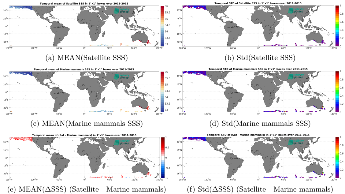
Figure 7: Temporal mean (left) and Std (right) of SSS from Aquarius SSS L3 CAP v5 - Monthly (JPL) (top), Marine mammals (middle), and of \Delta SSS (Satellite - Marine mammals). Only match-up pairs are used to generate these maps.
