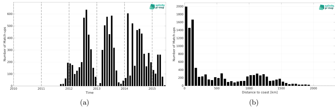
Figure 2: Number of match-ups between Marine mammals and Aquarius SSS L3 CAP v5 - Monthly (JPL) SSS as a function of time (a) and as function of the distance to coast (b) over the Mid-Low Latitudes 45N-45S Pi-MEP region and for the full satellite product period.
