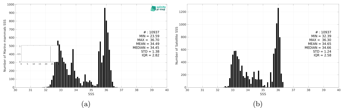
Figure 3: Histograms of SSS from Marine mammals (a) and Aquarius SSS L3 CAP v5 - Monthly (JPL) (b) considering all match-up pairs per bins of 0.1 over the Mid-Low Latitudes 45N-45S Pi-MEP region and for the full satellite product period.
