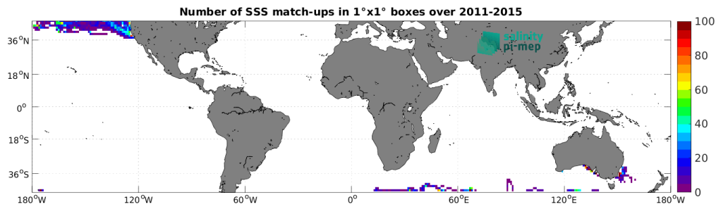
Figure 5: Number of SSS match-ups between Marine mammals SSS and the Aquarius SSS L3 CAP v5 - Monthly (JPL) SSS product for the Mid-Low Latitudes 45N-45S Pi-MEP region over 1^\circ \times 1^\circ boxes and for the full satellite product period.
