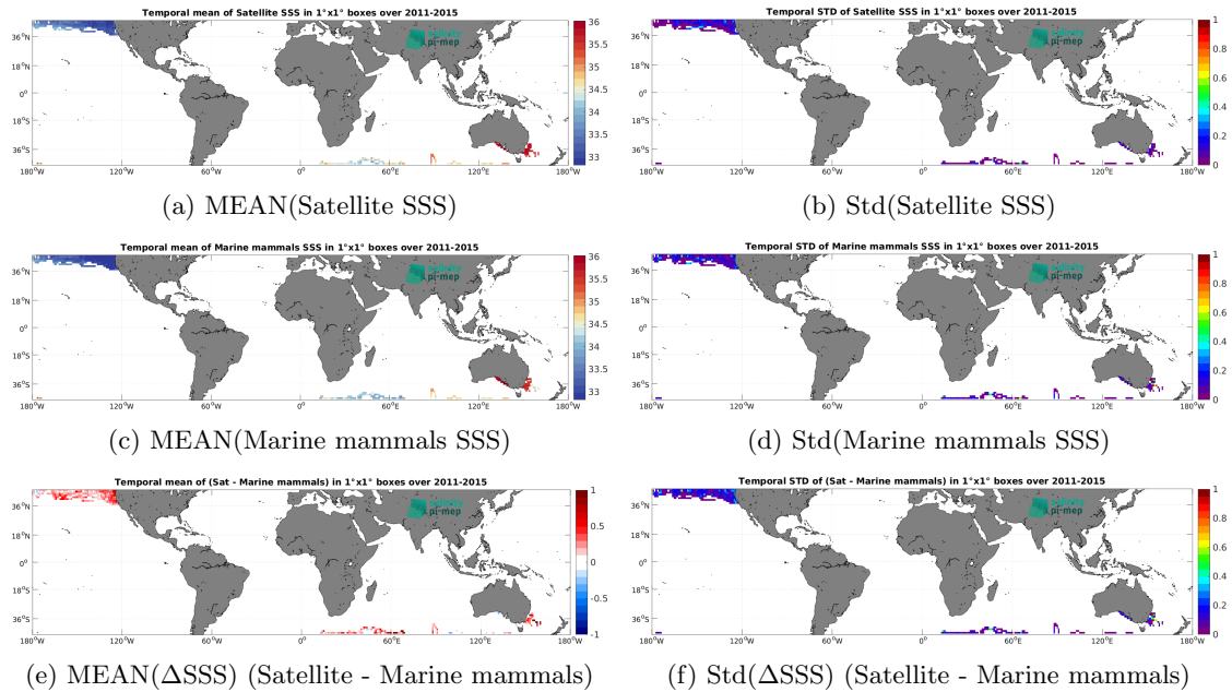
Figure 6: Temporal mean (left) and Std (right) of SSS from Aquarius SSS L3 CAP v5 - Monthly (JPL) (top), Marine mammals (middle), and of \Delta SSS (Satellite - Marine mammals). Only match-up pairs are used to generate these maps.
