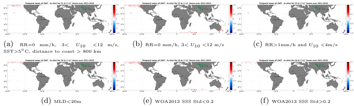
Figure 12: Temporal mean gridded over spatial boxes of size 1^\circ \times 1^\circ of \Delta SSS (Aquarius SSS L3 CAP v5 - Monthly (JPL) - Marine mammals) for 6 different subdatasets corresponding to: RR=0 mm/h, 3 < U_{10} < 12 m/s, SST > 5°C, distance to coast > 800 km (a), RR=0 mm/h, 3 < U_{10} < 12 m/s (b), RR > 1mm/h and U_{10} < 4 m/s (c), MLD < 20m (d), WOA2013 SSS Std < 0.2 (e), WOA2013 SSS Std > 0.2 (f).
