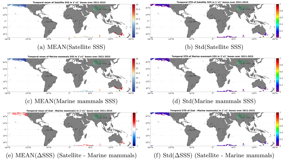
Figure 6: Temporal mean (left) and Std (right) of SSS from Aquarius SSS L3 CAP v5 - Monthly (JPL) (top), Marine mammals (middle), and of \Delta SSS (Satellite - Marine mammals). Only match-up pairs are used to generate these maps.
