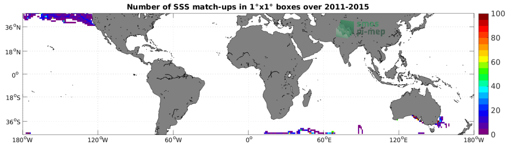
Figure 4: Number of SSS match-ups between Marine mammals SSS and the Aquarius SSS L3 CAP v5 - Monthly (JPL) SSS product for the Mid-Low Latitudes 45N-45S Pi-MEP region over 1^\circ \times 1^\circ boxes and for the full satellite product period.
