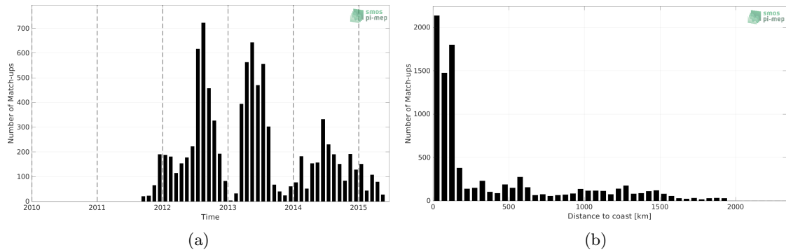
Figure 1: Number of match-ups between Marine mammals and Aquarius SSS L3 CAP v5 - Monthly (JPL) SSS as a function of time (a) and as function of the distance to coast (b) over the Mid-Low Latitudes 45N-45S Pi-MEP region and for the full satellite product period.
