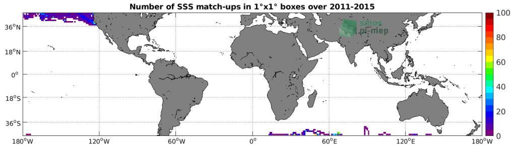
Figure 4: Number of SSS match-ups between Sea mammals SSS and the Aquarius SSS L3 CAP v5 - Monthly (JPL) SSS product for the Mid-Low Latitudes 45N-45S Pi-MEP region over 1^\circ \times 1^\circ boxes and for the full satellite product period.
