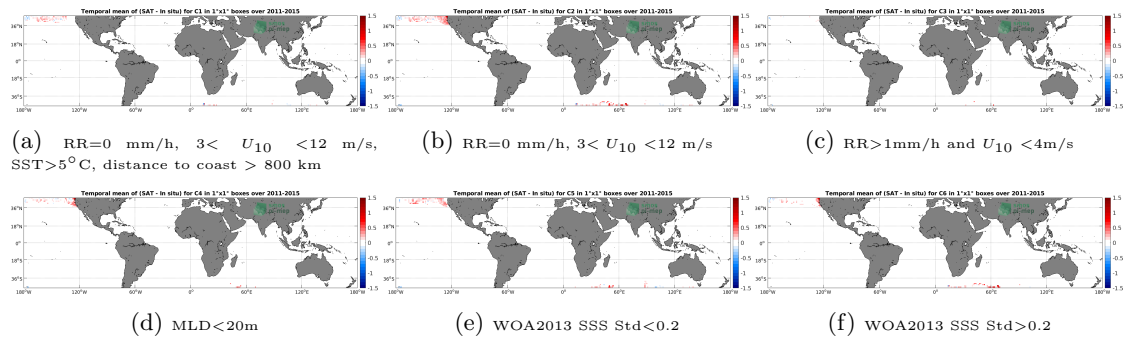
Figure 12: Temporal mean gridded over spatial boxes of size 1^\circ \times 1^\circ of \Delta SSS (Aquarius SSS L3 CAP v5 - Monthly (JPL) - Sea mammals) for 6 different subdatasets corresponding to:RR=0 mm/h, 3 < U_{10} < 12 m/s, SST >5^\circ C, distance to coast > 800 km (a), RR=0 mm/h, 3 < U_{10} < 12 m/s (b), RR >1 mm/h and U_{10} < 4 m/s (c),MLD <20 m (d),WOA2013 SSS Std <0.2 (e),WOA2013 SSS Std >0.2 (f).
