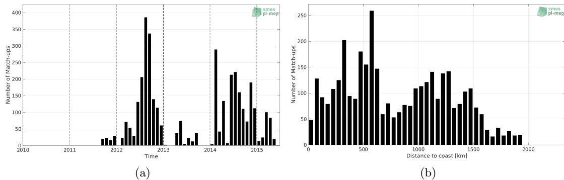
Figure 1: Number of match-ups between Sea mammals and Aquarius SSS L3 CAP v5 - Monthly (JPL) SSS as a function of time (a) and as function of the distance to coast (b) over the Mid-Low Latitudes 45N-45S Pi-MEP region and for the full satellite product period.
