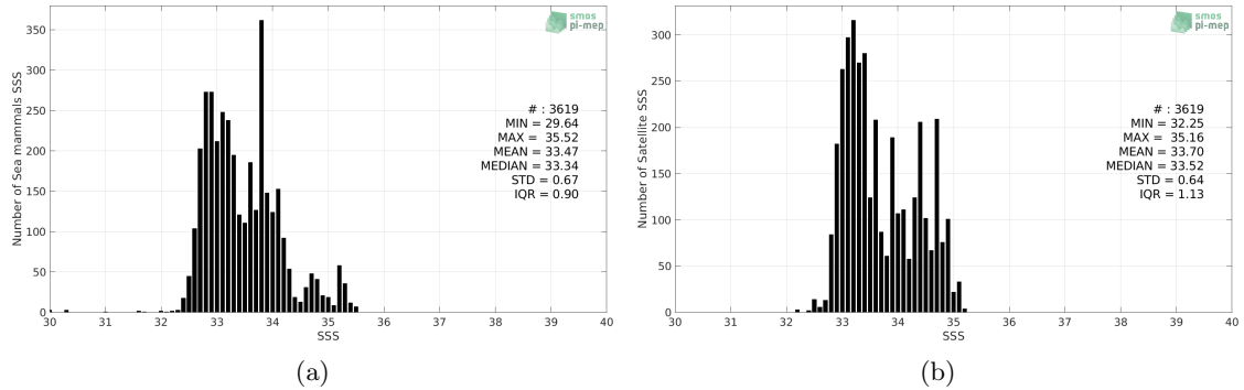
Figure 2: Histograms of SSS from Sea mammals (a) and Aquarius SSS L3 CAP v5 - Monthly (JPL) (b) considering all match-up pairs per bins of 0.1 over the Mid-Low Latitudes 45N-45S Pi-MEP region and for the full satellite product period.
