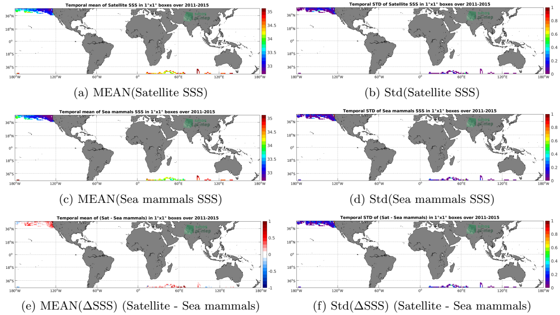
Figure 6: Temporal mean (left) and Std (right) of SSS from Aquarius SSS L3 CAP v5 - Monthly (JPL) (top), Sea mammals (middle), and of \Delta SSS (Satellite - Sea mammals). Only match-up pairs are used to generate these maps.
