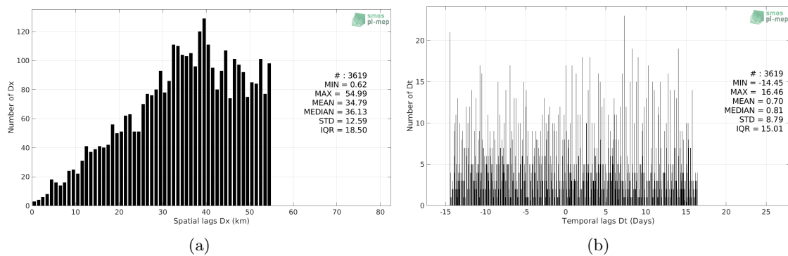
Figure 5: Histograms of the spatial (a) and temporal (b) lags between the location/time of the Sea mammals measurement and the date of the corresponding Aquarius SSS L3 CAP v5 - Monthly (JPL) SSS pixel.
