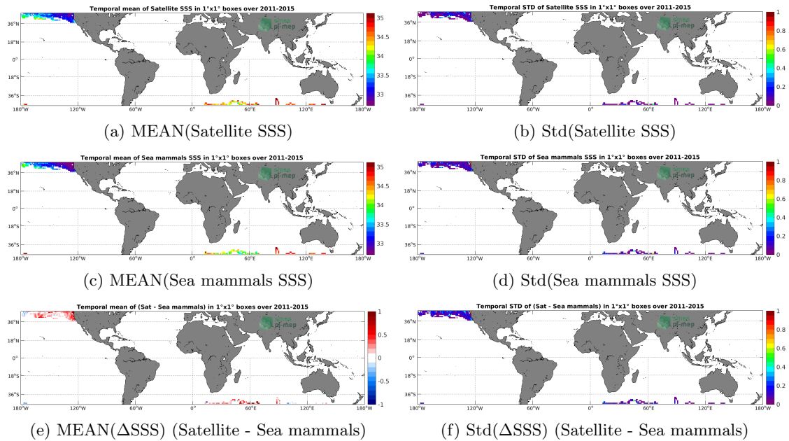
Figure 6: Temporal mean (left) and Std (right) of SSS from Aquarius SSS L3 CAP v5 - Monthly (JPL) (top), Sea mammals (middle), and of \Delta SSS (Satellite - Sea mammals). Only match-up pairs are used to generate these maps.
