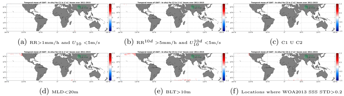
Figure 12: Temporal mean gridded over spatial boxes of size 1°x1° of \Delta SSS (Aquarius-L3-JPL-V5-MONTHLY - Sea mammals) for 6 different subdatasets corresponding to: RR>1mm/h and U_{10} < 5m/s (a), RR^{10d} > 5mm/h and U_{10}^{10d} < 5m/s (b), C1 U C2 (c),MLD<20m (d),BLT>10m (e),Locations where WOA2013 SSS STD>0.2 (f).
