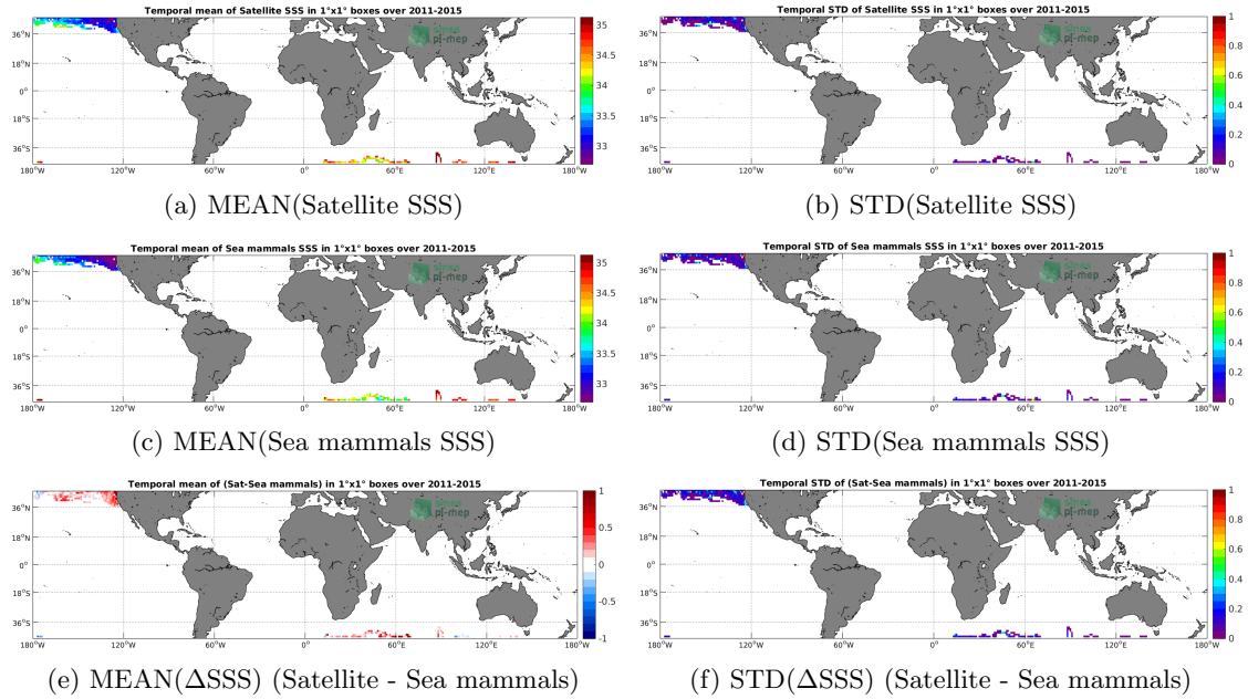
Figure 6: Temporal mean (left) and STD (right) of SSS from Aquarius-L3-JPL-V5-MONTHLY (top), Sea mammals (middle), and of \Delta SSS (Satellite - Sea mammals). Only match-up pairs are used to generate these maps.
