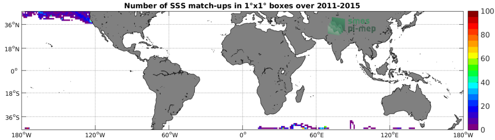
Figure 4: Number of SSS match-ups between Sea mammals SSS and the Aquarius-L3-JPL-V5-MONTHLY SSS product for the Mid-Low Latitudes 45N-45S Pi-MEP region over 1^\circ \times 1^\circ boxes and for the full satellite product period.
