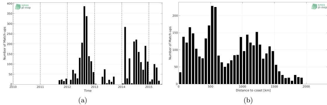
Figure 1: Number of match-ups between Sea mammals and Aquarius-L3-JPL-V5-MONTHLY SSS as a function of time (a) and as function of the distance to coast (b) over the Mid-Low Latitudes 45N-45S Pi-MEP region and for the full satellite product period.
