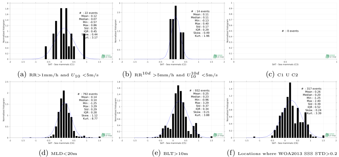
Figure 13: Normalized histogram of \Delta SSS (Aquarius-L3-JPL-V5-MONTHLY - Sea mammals) for 6 different subdatasets corresponding to: RR>1mm/h and U_{10} < 5m/s (a), RR^{10d} > 5mm/h and U_{10}^{10d} < 5m/s (b), C1 U C2 (c),MLD<20m (d),BLT>10m (e),Locations where WOA2013 SSS STD>0.2 (f).
