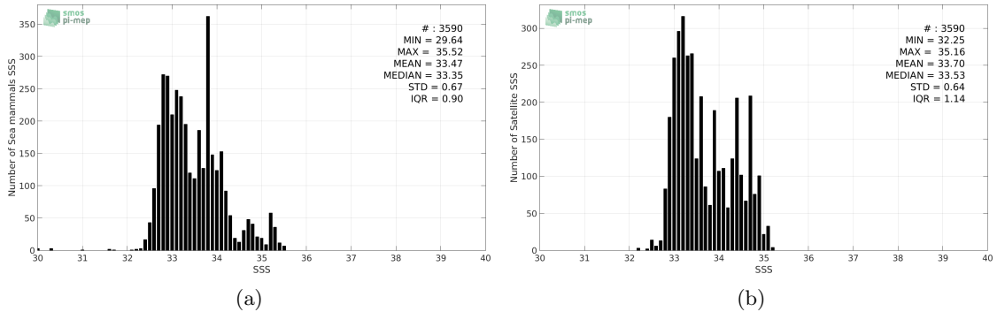
Figure 2: Histograms of SSS from Sea mammals (a) and Aquarius-L3-JPL-V5-MONTHLY (b) considering all match-up pairs per bins of 0.1 over the Mid-Low Latitudes 45N-45S Pi-MEP region and for the full satellite product period.
