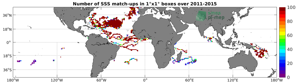
Figure 3: Number of SSS match-ups between Surface drifters SSS and the Aquarius SSS L3 CAP v5 - Monthly (JPL) SSS product for the Mid-Low Latitudes 45N-45S Pi-MEP region over 1°x1° boxes and for the full satellite product period.
