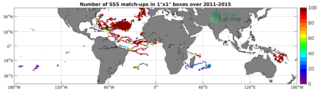
Figure 3: Number of SSS match-ups between Surface drifters SSS and the Aquarius-L3-JPL-V5-MONTHLY SSS product for the Mid-Low Latitudes 45N-45S Pi-MEP region over 1°x1° boxes and for the full satellite product period.
