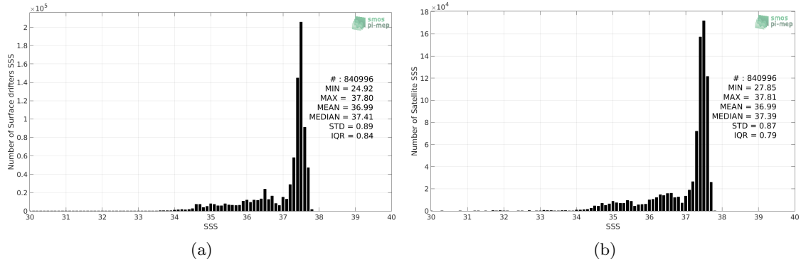
Figure 2: Histograms of SSS from Surface drifters (a) and Aquarius-L3-JPL-V5-MONTHLY (b) considering all match-up pairs per bins of 0.1 over the Mid-Low Latitudes 45N-45S Pi-MEP region and for the full satellite product period.
