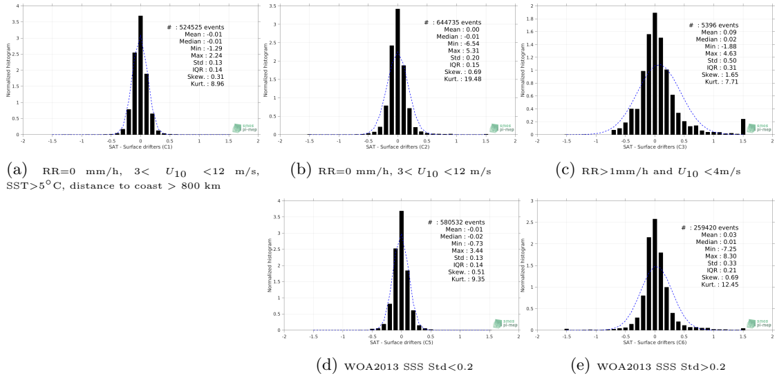
Figure 12: Normalized histogram of \Delta SSS (Aquarius-L3-JPL-V5-MONTHLY - Surface drifters) for 5 different subdatasets corresponding to: RR=0 mm/h, 3 < U_{10} < 12 m/s, SST >5^\circ\text{C} , distance to coast > 800 km (a), RR=0 mm/h, 3 < U_{10} < 12 m/s (b), RR >1 mm/h and U_{10} < 4 m/s (c), WOA2013 SSS Std <0.2 (d), WOA2013 SSS Std >0.2 (e).
