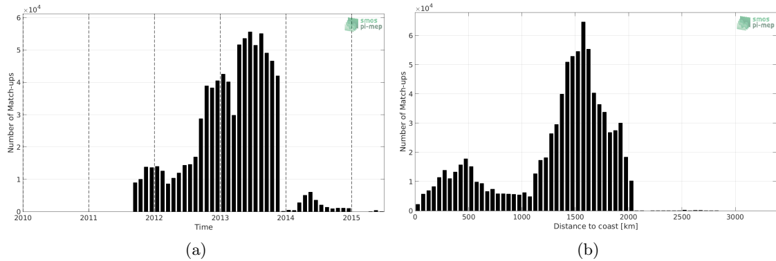
Figure 1: Number of match-ups between Surface drifters and Aquarius-L3-JPL-V5-MONTHLY SSS as a function of time (a) and as function of the distance to coast (b) over the Mid-Low Latitudes 45N-45S Pi-MEP region and for the full satellite product period.
