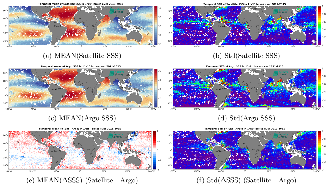
Figure 6: Temporal mean (left) and Std (right) of SSS from Aquarius SSS L3 CAP v5 - Monthly (JPL) (top), Argo (middle), and of \Delta SSS (Satellite - Argo). Only match-up pairs are used to generate these maps.
