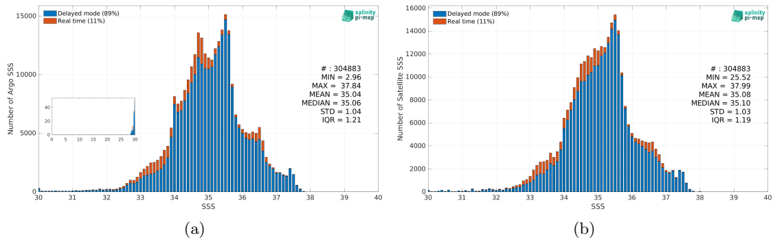
Figure 2: Histograms of SSS from Argo (a) and Aquarius SSS L3 CAP v5 - Monthly (JPL) (b) considering all match-up pairs per bins of 0.1 over the Mid-Low Latitudes 45N-45S Pi-MEP region and for the full satellite product period.
