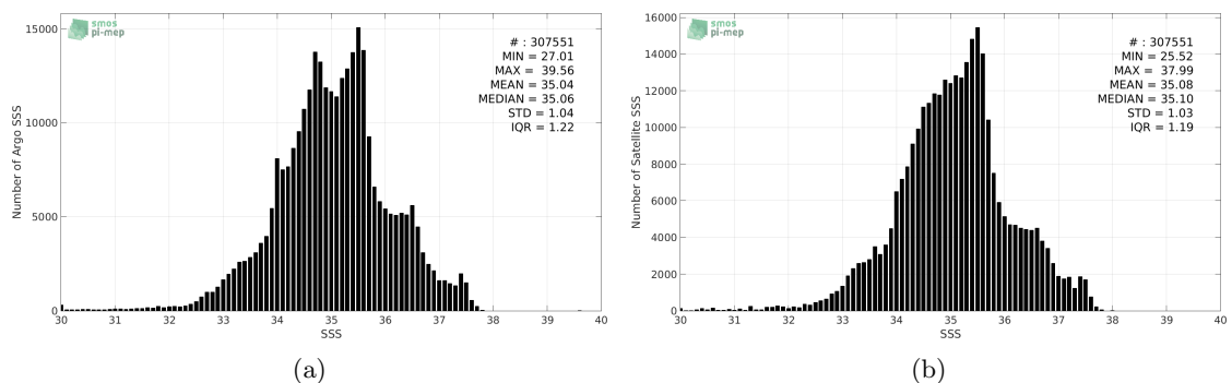
Figure 2: Histograms of SSS from Argo (a) and Aquarius-L3-JPL-V5-MONTHLY (b) considering all match-up pairs per bins of 0.1 over the Mid-Low Latitudes 45N-45S Pi-MEP region and for the full satellite product period.
