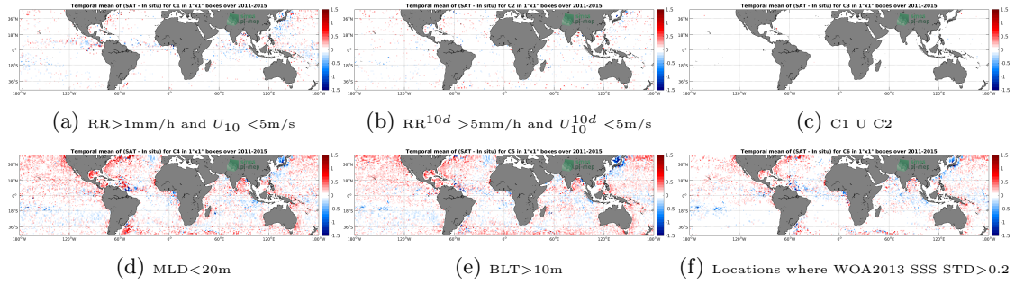
Figure 12: Temporal mean gridded over spatial boxes of size 1°x1° of \Delta SSS (Aquarius-L3-JPL-V5-MONTHLY - Argo) for 6 different subdatasets corresponding to:RR>1mm/h and U_{10} < 5m/s (a), RR^{10d} > 5mm/h and U_{10}^{10d} < 5m/s (b), C1 U C2 (c),MLD<20m (d),BLT>10m (e),Locations where WOA2013 SSS STD>0.2 (f).
