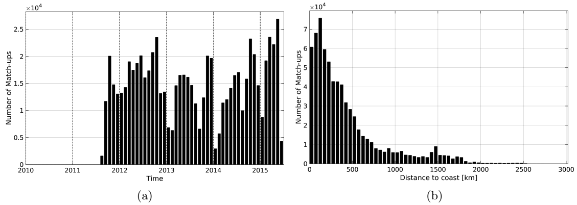
Figure 1: Number of match-ups between TSG-LEGOS-DM and Aquarius-L3-JPL-V4-7DAY-RUNNING SSS as a function of time (a) and as function of the distance to coast (b) over the Mid-Low Latitudes 45N-45S Pi-MEP region and for the full satellite product period.
