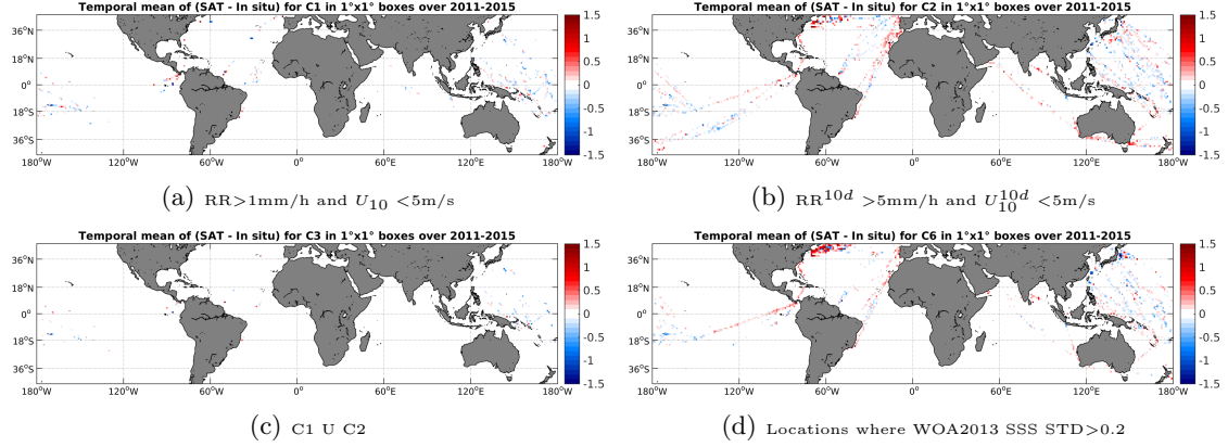
Figure 12: Temporal mean gridded over spatial boxes of size 1^\circ \times 1^\circ of \Delta SSS (Aquarius-L3-JPL-V4-7DAY-RUNNING - TSG-LEGOS-DM) for 4 different subdatasets corresponding to: RR > 1\text{mm/h} and U_{10} < 5\text{m/s} (a), RR^{10d} > 5\text{mm/h} and U_{10}^{10d} < 5\text{m/s} (b), C1 U C2 (c), Locations where WOA2013 SSS STD > 0.2 (d).
