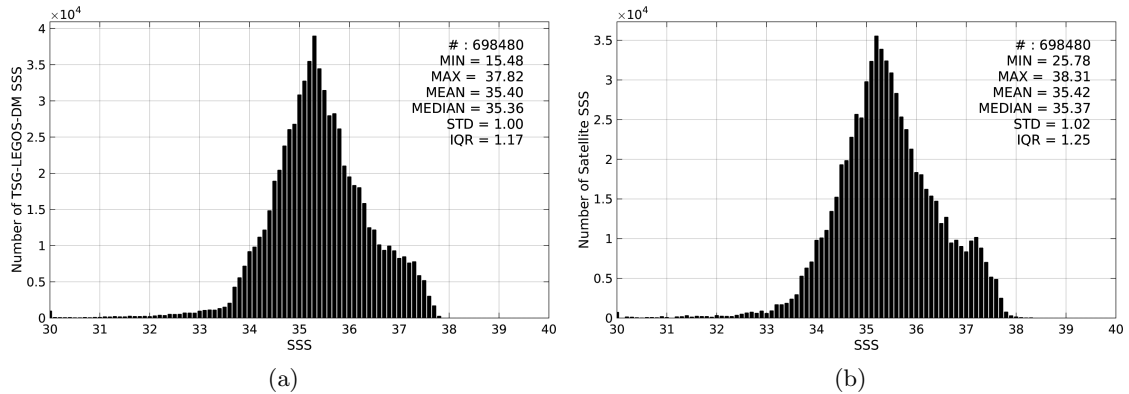
Figure 2: Histograms of SSS from TSG-LEGOS-DM (a) and Aquarius-L3-JPL-V4-7DAY-RUNNING (b) considering all match-up pairs per bins of 0.1 over the Mid-Low Latitudes 45N-45S Pi-MEP region and for the full satellite product period.
