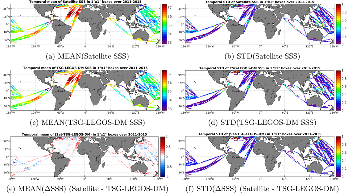
Figure 6: Temporal mean (left) and STD (right) of SSS from Aquarius-L3-JPL-V4-7DAY-RUNNING (top), TSG-LEGOS-DM (middle), and of \Delta SSS (Satellite - TSG-LEGOS-DM). Only match-up pairs are used to generate these maps.
