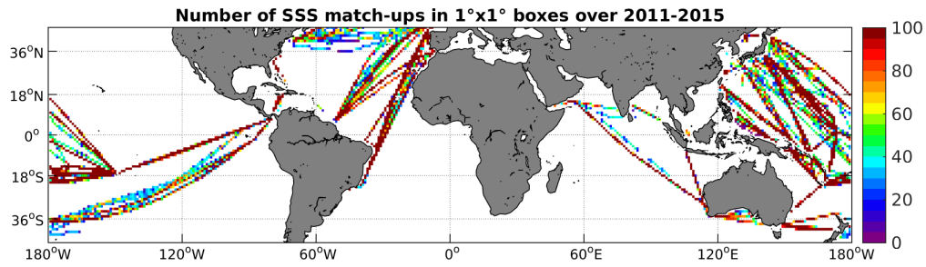
Figure 4: Number of SSS match-ups between TSG-LEGOS-DM SSS and the Aquarius-L3-JPL-V4-7DAY-RUNNING SSS product for the Mid-Low Latitudes 45N-45S Pi-MEP region over 1^\circ \times 1^\circ boxes and for the full satellite product period.
