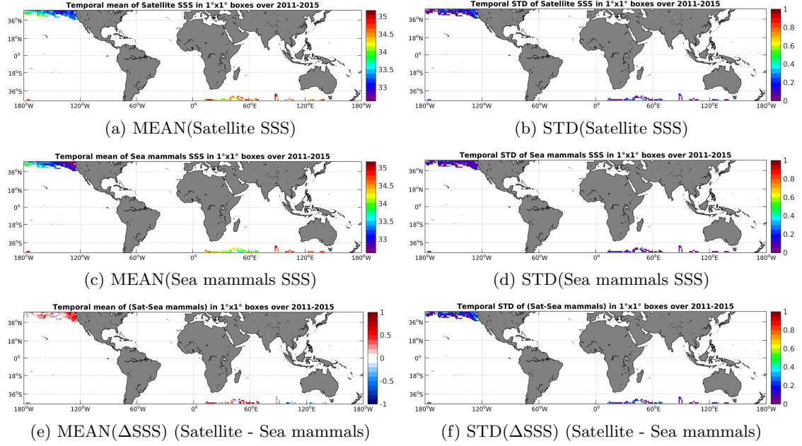
Figure 6: Temporal mean (left) and STD (right) of SSS from Aquarius-L3-JPL-V4-7DAY-RUNNING (top), Sea mammals (middle), and of \Delta SSS (Satellite - Sea mammals). Only match-up pairs are used to generate these maps.
