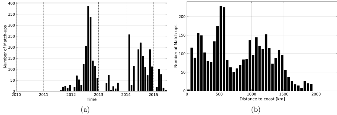
Figure 1: Number of match-ups between Sea mammals and Aquarius-L3-JPL-V4-7DAY-RUNNING SSS as a function of time (a) and as function of the distance to coast (b) over the Mid-Low Latitudes 45N-45S Pi-MEP region and for the full satellite product period.
