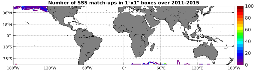
Figure 4: Number of SSS match-ups between Sea mammals SSS and the Aquarius-L3-JPL-V4-7DAY-RUNNING SSS product for the Mid-Low Latitudes 45N-45S Pi-MEP region over 1^\circ \times 1^\circ boxes and for the full satellite product period.
