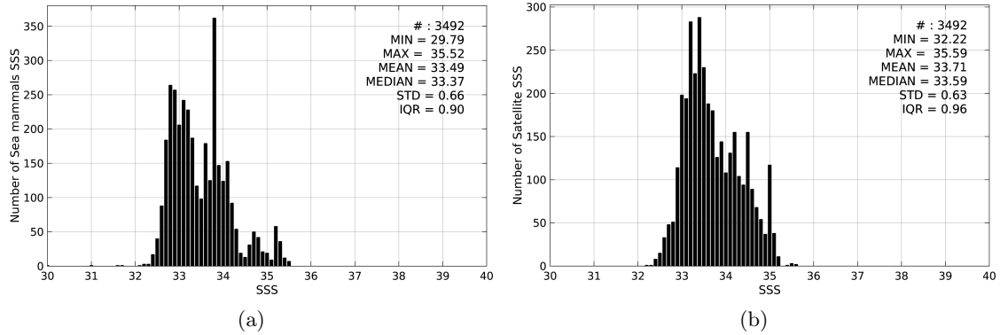
Figure 2: Histograms of SSS from Sea mammals (a) and Aquarius-L3-JPL-V4-7DAY-RUNNING (b) considering all match-up pairs per bins of 0.1 over the Mid-Low Latitudes 45N-45S Pi-MEP region and for the full satellite product period.
