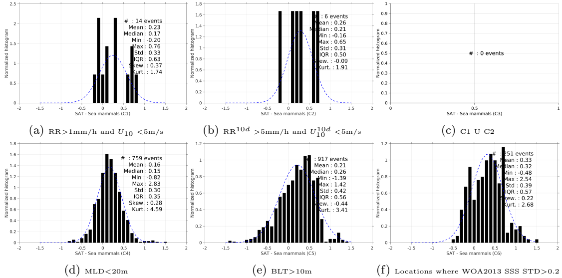
Figure 13: Normalized histogram of \Delta SSS (Aquarius-L3-JPL-V4-7DAY-RUNNING - Sea mammals) for 6 different subdatasets corresponding to: RR > 1\text{mm/h} and U_{10} < 5\text{m/s} (a), RR^{10d} > 5\text{mm/h} and U_{10}^{10d} < 5\text{m/s} (b), C1 U C2 (c), MLD < 20\text{m} (d), BLT > 10\text{m} (e), Locations where WOA2013 SSS STD > 0.2 (f).
