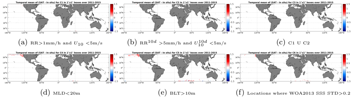
Figure 12: Temporal mean gridded over spatial boxes of size 1^\circ \times 1^\circ of \Delta SSS (Aquarius-L3-JPL-V4-7DAY-RUNNING - Sea mammals) for 6 different subdatasets corresponding to: RR > 1\text{mm/h} and U_{10} < 5\text{m/s} (a), RR^{10d} > 5\text{mm/h} and U_{10}^{10d} < 5\text{m/s} (b), C1 U C2 (c), MLD < 20\text{m} (d), BLT > 10\text{m} (e), Locations where WOA2013 SSS STD > 0.2 (f).
