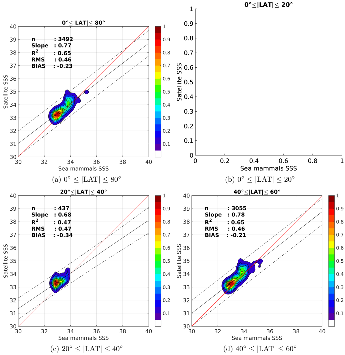
Figure 9: Contour maps of the concentration of Aquarius-L3-JPL-V4-7DAY-RUNNING SSS (y-axis) versus Sea mammals SSS (x-axis) at match-up pairs for different latitude bands. For each plot, the red line shows x=y . The black thin and dashed lines indicate a linear fit through the data cloud and the \pm 95\% confidence levels, respectively. The number match-up pairs n , the slope and R^2 coefficient of the linear fit, the root mean square (RMS) and the mean bias between satellite and in situ data are indicated for each latitude band in each plots.
