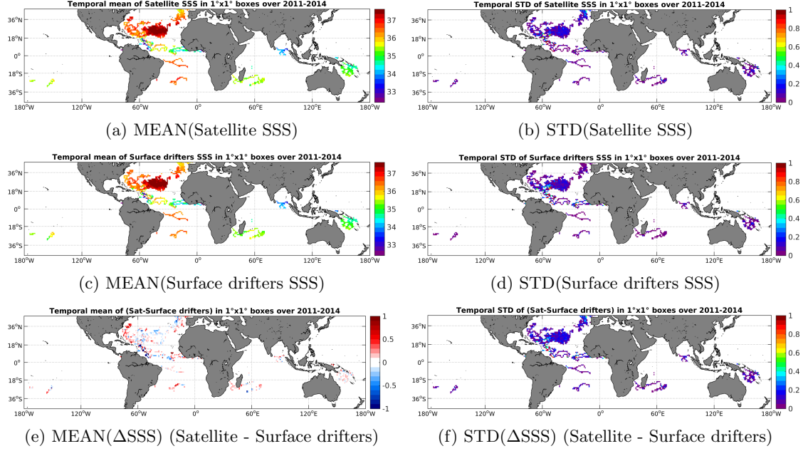
Figure 5: Temporal mean (left) and STD (right) of SSS from Aquarius-L3-JPL-V4-7DAY-RUNNING (top), Surface drifters (middle), and of \Delta SSS (Satellite - Surface drifters). Only match-up pairs are used to generate these maps.
