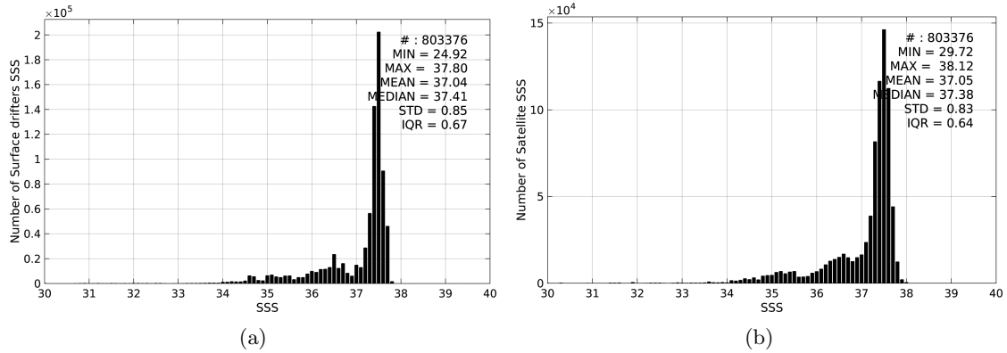
Figure 2: Histograms of SSS from Surface drifters (a) and Aquarius-L3-JPL-V4-7DAY-RUNNING (b) considering all match-up pairs per bins of 0.1 over the Mid-Low Latitudes 45N-45S Pi-MEP region and for the full satellite product period.
