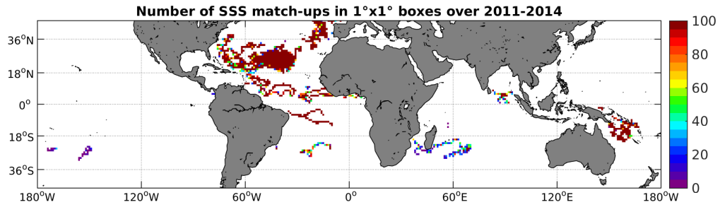
Figure 3: Number of SSS match-ups between Surface drifters SSS and the Aquarius-L3-JPL-V4-7DAY-RUNNING SSS product for the Mid-Low Latitudes 45N-45S Pi-MEP region over 1°x1° boxes and for the full satellite product period.
