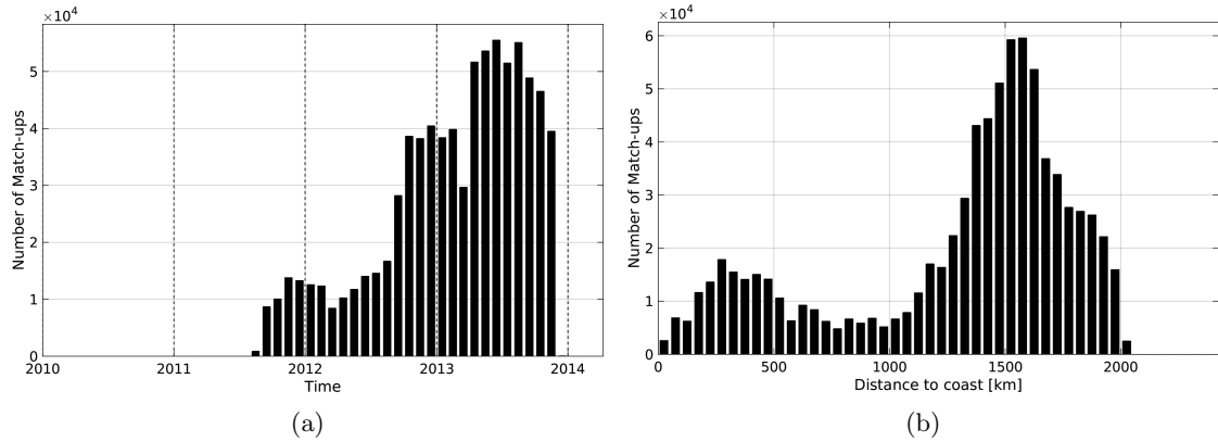
Figure 1: Number of match-ups between Surface drifters and Aquarius-L3-JPL-V4-7DAY-RUNNING SSS as a function of time (a) and as function of the distance to coast (b) over the Mid-Low Latitudes 45N-45S Pi-MEP region and for the full satellite product period.
