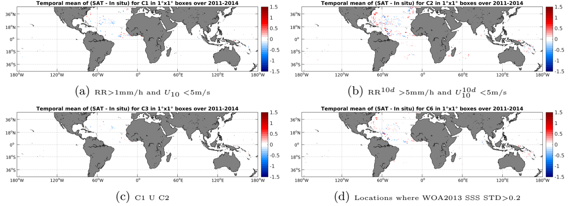
Figure 11: Temporal mean gridded over spatial boxes of size 1^\circ \times 1^\circ of \Delta SSS (Aquarius-L3-JPL-V4-7DAY-RUNNING - Surface drifters) for 4 different subdatasets corresponding to: RR > 1\text{mm/h} and U_{10} < 5\text{m/s} (a), RR^{10d} > 5\text{mm/h} and U_{10}^{10d} < 5\text{m/s} (b), C1 U C2 (c), Locations where WOA2013 SSS STD > 0.2 (d).
