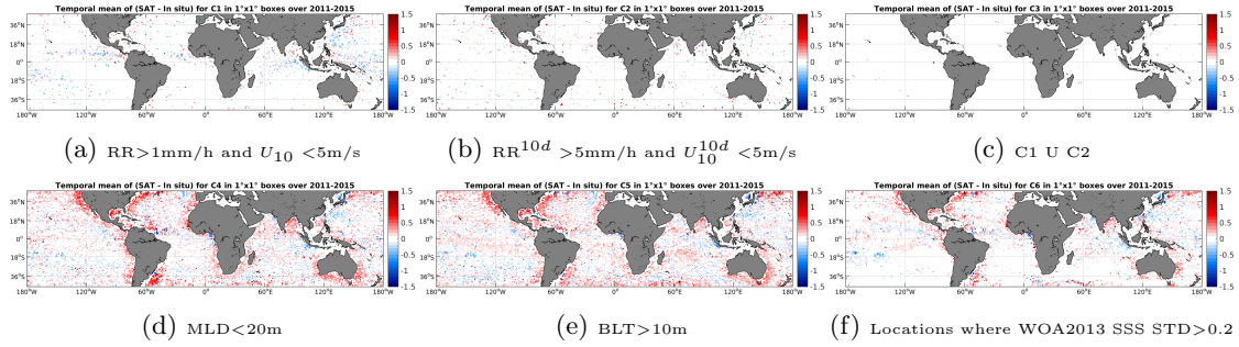
Figure 12: Temporal mean gridded over spatial boxes of size 1^\circ \times 1^\circ of \Delta SSS (Aquarius-L3-JPL-V4-7DAY-RUNNING - Argo) for 6 different subdatasets corresponding to: RR > 1\text{mm/h} and U_{10} < 5\text{m/s} (a), RR^{10d} > 5\text{mm/h} and U_{10}^{10d} < 5\text{m/s} (b), C1 U C2 (c), MLD < 20\text{m} (d), BLT > 10\text{m} (e), Locations where WOA2013 SSS STD > 0.2 (f).
