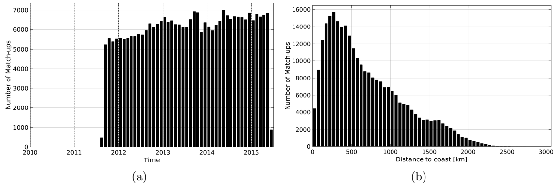
Figure 1: Number of match-ups between Argo and Aquarius-L3-JPL-V4-7DAY-RUNNING SSS as a function of time (a) and as function of the distance to coast (b) over the Mid-Low Latitudes 45N-45S Pi-MEP region and for the full satellite product period.
