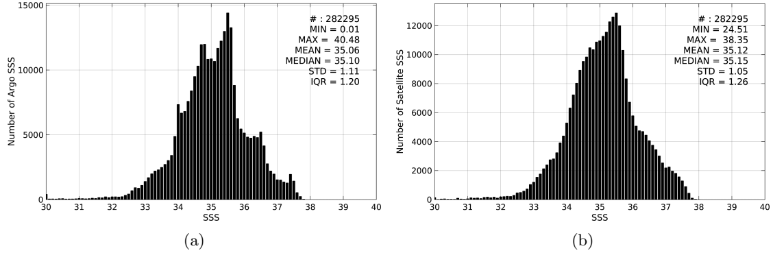
Figure 2: Histograms of SSS from Argo (a) and Aquarius-L3-JPL-V4-7DAY-RUNNING (b) considering all match-up pairs per bins of 0.1 over the Mid-Low Latitudes 45N-45S Pi-MEP region and for the full satellite product period.
