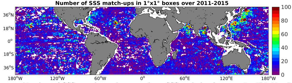
Figure 4: Number of SSS match-ups between Argo SSS and the Aquarius-L3-JPL-V4-7DAY-RUNNING SSS product for the Mid-Low Latitudes 45N-45S Pi-MEP region over 1^\circ \times 1^\circ boxes and for the full satellite product period.
