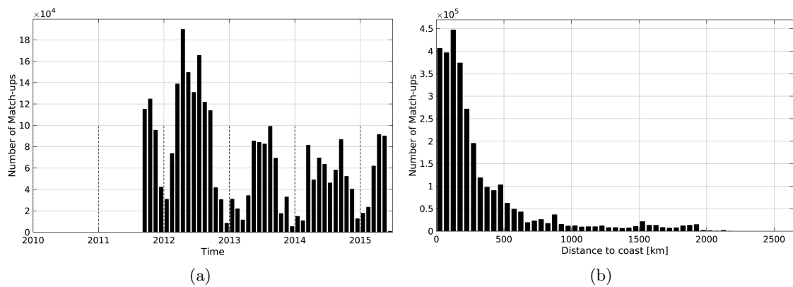
Figure 1: Number of match-ups between TSG-SAMOS and Aquarius-L3-JPL-V4-MONTHLY SSS as a function of time (a) and as function of the distance to coast (b) over the Mid-Low Latitudes 45N-45S Pi-MEP region and for the full satellite product period.
