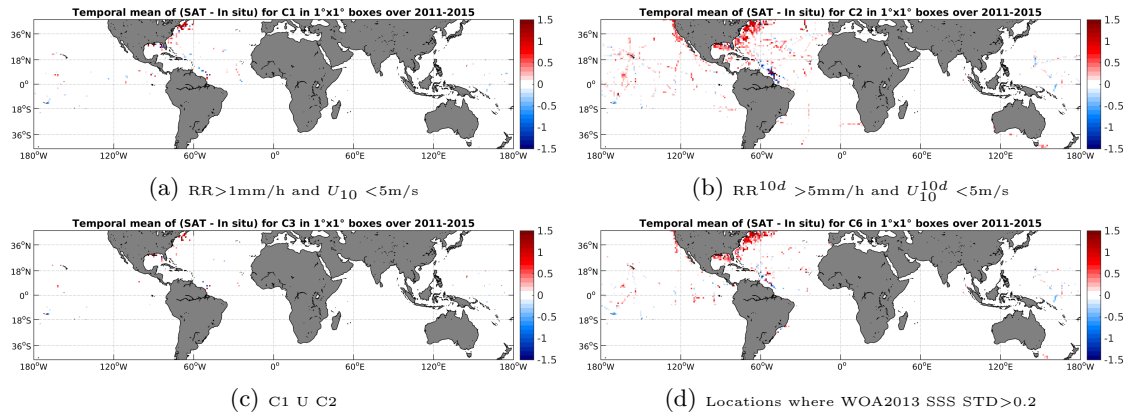
Figure 12: Temporal mean gridded over spatial boxes of size 1^\circ \times 1^\circ of \Delta SSS (Aquarius-L3-JPL-V4-MONTHLY - TSG-SAMOS) for 4 different subdatasets corresponding to: RR > 1\text{mm/h} and U_{10} < 5\text{m/s} (a), RR^{10d} > 5\text{mm/h} and U_{10}^{10d} < 5\text{m/s} (b), C1 U C2 (c), Locations where WOA2013 SSS STD > 0.2 (d).
