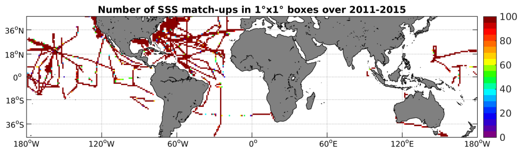
Figure 4: Number of SSS match-ups between TSG-SAMOS SSS and the Aquarius-L3-JPL-V4-MONTHLY SSS product for the Mid-Low Latitudes 45N-45S Pi-MEP region over 1°x1° boxes and for the full satellite product period.
