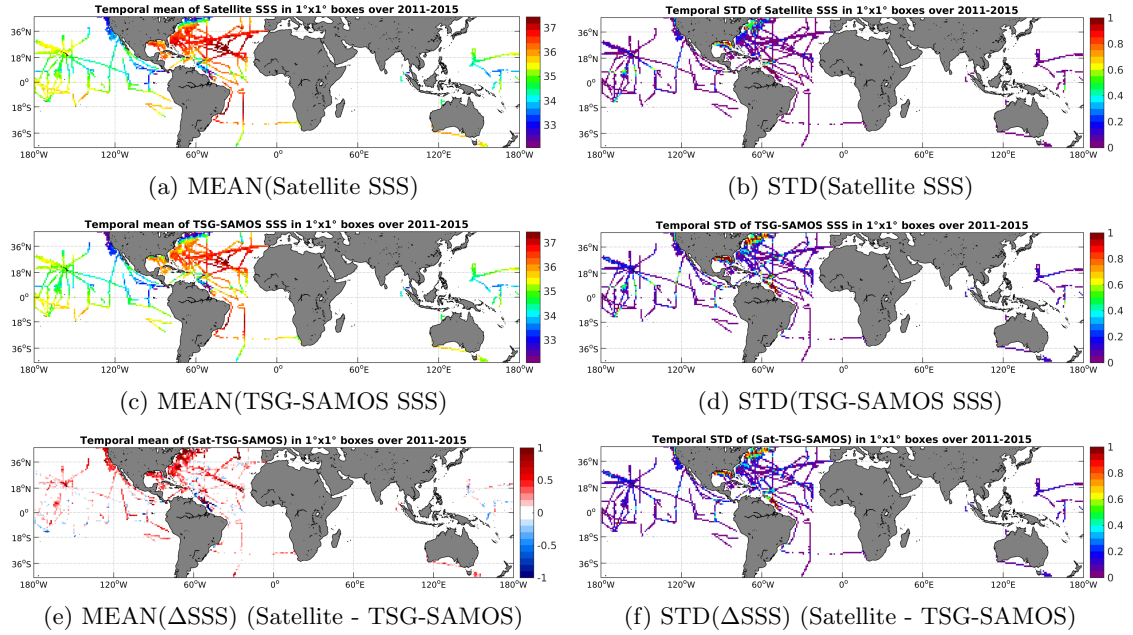
Figure 6: Temporal mean (left) and STD (right) of SSS from Aquarius-L3-JPL-V4-MONTHLY (top), TSG-SAMOS (middle), and of \Delta SSS (Satellite - TSG-SAMOS). Only match-up pairs are used to generate these maps.
