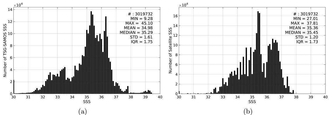
Figure 2: Histograms of SSS from TSG-SAMOS (a) and Aquarius-L3-JPL-V4-MONTHLY (b) considering all match-up pairs per bins of 0.1 over the Mid-Low Latitudes 45N-45S Pi-MEP region and for the full satellite product period.
