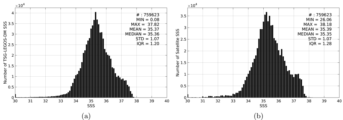
Figure 2: Histograms of SSS from TSG-LEGOS-DM (a) and Aquarius-L3-JPL-V4-MONTHLY (b) considering all match-up pairs per bins of 0.1 over the Mid-Low Latitudes 45N-45S Pi-MEP region and for the full satellite product period.
