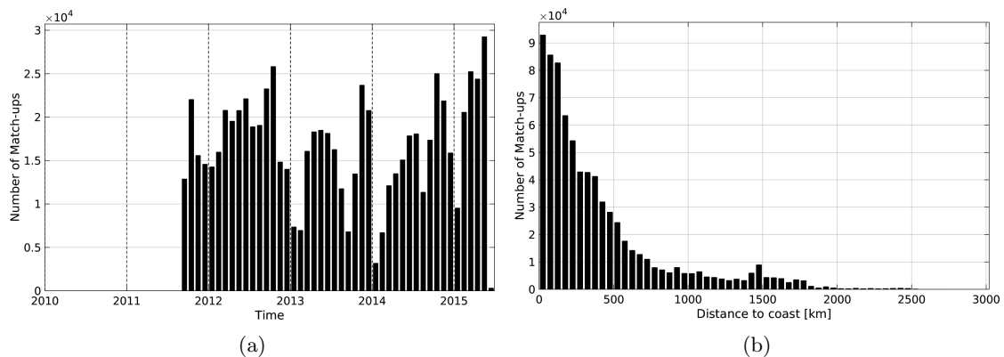
Figure 1: Number of match-ups between TSG-LEGOS-DM and Aquarius-L3-JPL-V4-MONTHLY SSS as a function of time (a) and as function of the distance to coast (b) over the Mid-Low Latitudes 45N-45S Pi-MEP region and for the full satellite product period.
