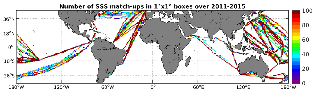
Figure 4: Number of SSS match-ups between TSG-LEGOS-DM SSS and the Aquarius-L3-JPL-V4-MONTHLY SSS product for the Mid-Low Latitudes 45N-45S Pi-MEP region over 1^\circ \times 1^\circ boxes and for the full satellite product period.
