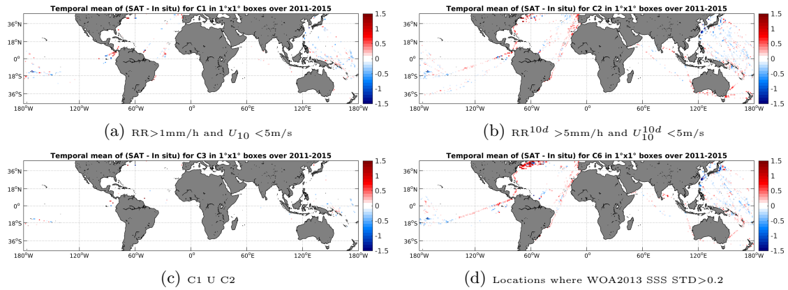
Figure 12: Temporal mean gridded over spatial boxes of size 1^\circ \times 1^\circ of \Delta SSS (Aquarius-L3-JPL-V4-MONTHLY - TSG-LEGOS-DM) for 4 different subdatasets corresponding to: RR > 1\text{mm/h} and U_{10} < 5\text{m/s} (a), RR^{10d} > 5\text{mm/h} and U_{10}^{10d} < 5\text{m/s} (b), C1 U C2 (c), Locations where WOA2013 SSS STD > 0.2 (d).
