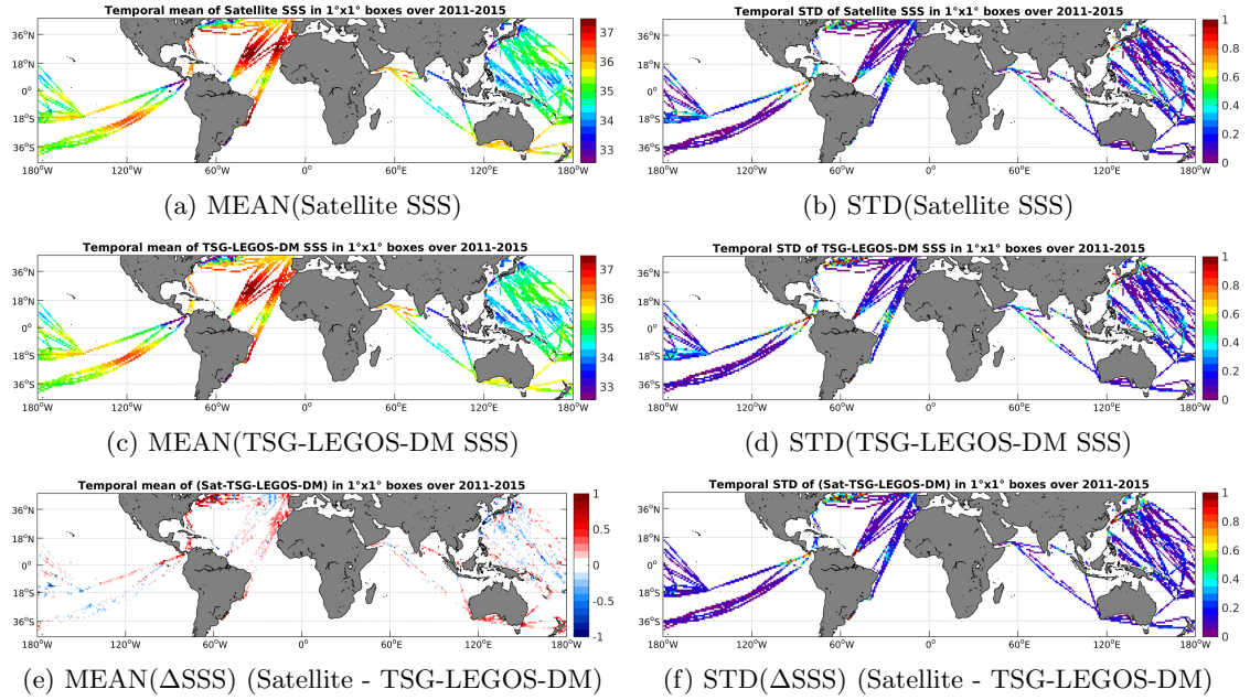
Figure 6: Temporal mean (left) and STD (right) of SSS from Aquarius-L3-JPL-V4-MONTHLY (top), TSG-LEGOS-DM (middle), and of \Delta SSS (Satellite - TSG-LEGOS-DM). Only match-up pairs are used to generate these maps.
