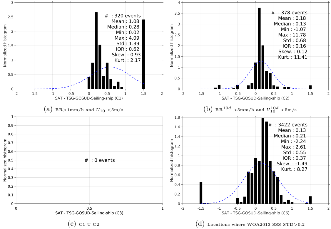
Figure 13: Normalized histogram of \Delta\text{SSS} (Aquarius-L3-JPL-V4-MONTHLY - TSG-GOSUD-Sailing-ship) for 6 different subdatasets corresponding to: RR > 1mm/h and U_{10} < 5\text{m/s} (a), RR^{10d} > 5\text{mm/h} and U_{10}^{10d} < 5\text{m/s} (b), C1 U C2 (c), Locations where WOA2013 SSS STD > 0.2 (d).
