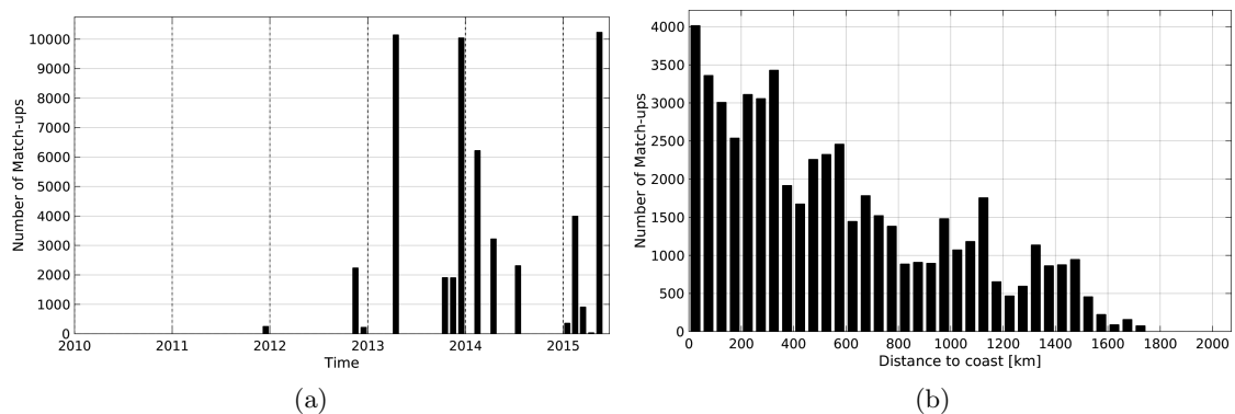
Figure 1: Number of match-ups between TSG-GOSUD-Sailing-ship and Aquarius-L3-JPL-V4-MONTHLY SSS as a function of time (a) and as function of the distance to coast (b) over the Mid-Low Latitudes 45N-45S Pi-MEP region and for the full satellite product period.
