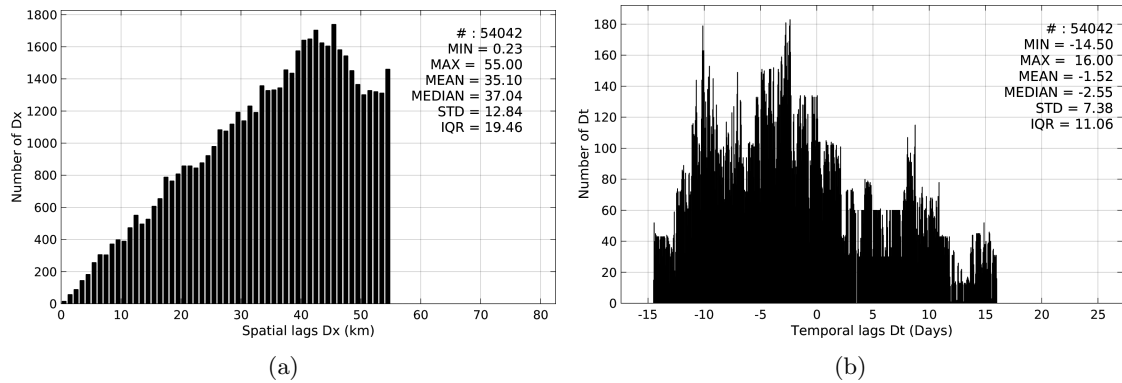
Figure 5: Histograms of the spatial (a) and temporal (b) lags between the time of the TSG-GOSUD-Sailing-ship measurements and the date of the corresponding Aquarius-L3-JPL-V4-MONTHLY SSS product.
