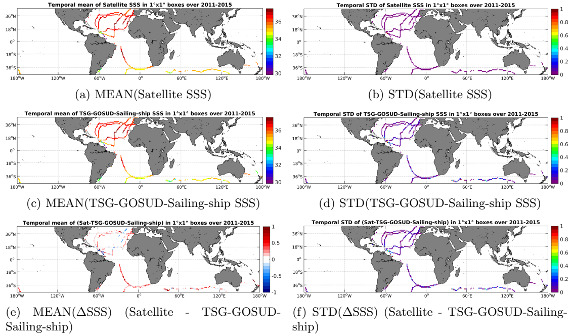
Figure 6: Temporal mean (left) and STD (right) of SSS from Aquarius-L3-JPL-V4-MONTHLY (top), TSG-GOSUD-Sailing-ship (middle), and of \Delta SSS (Satellite - TSG-GOSUD-Sailing-ship). Only match-up pairs are used to generate these maps.
