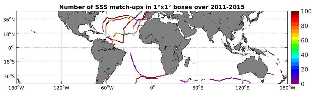
Figure 4: Number of SSS match-ups between TSG-GOSUD-Sailing-ship SSS and the Aquarius-L3-JPL-V4-MONTHLY SSS product for the Mid-Low Latitudes 45N-45S Pi-MEP region over 1^\circ \times 1^\circ boxes and for the full satellite product period.
