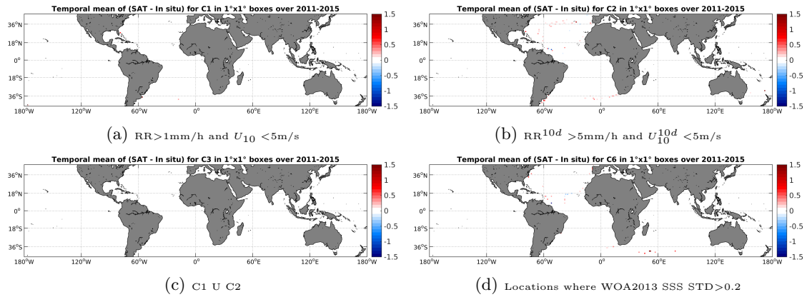
Figure 12: Temporal mean gridded over spatial boxes of size 1^\circ \times 1^\circ of \Delta SSS (Aquarius-L3-JPL-V4-MONTHLY - TSG-GOSUD-Sailing-ship) for 4 different subdatasets corresponding to: RR > 1\text{mm/h} and U_{10} < 5\text{m/s} (a), RR^{10d} > 5\text{mm/h} and U_{10}^{10d} < 5\text{m/s} (b), C1 U C2 (c), Locations where WOA2013 SSS STD > 0.2 (d).
