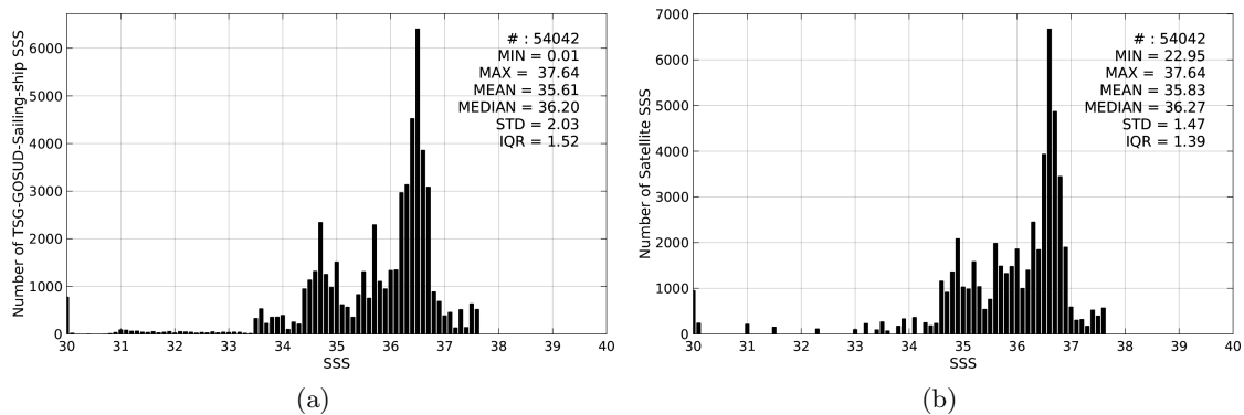
Figure 2: Histograms of SSS from TSG-GOSUD-Sailing-ship (a) and Aquarius-L3-JPL-V4-MONTHLY (b) considering all match-up pairs per bins of 0.1 over the Mid-Low Latitudes 45N-45S Pi-MEP region and for the full satellite product period.
