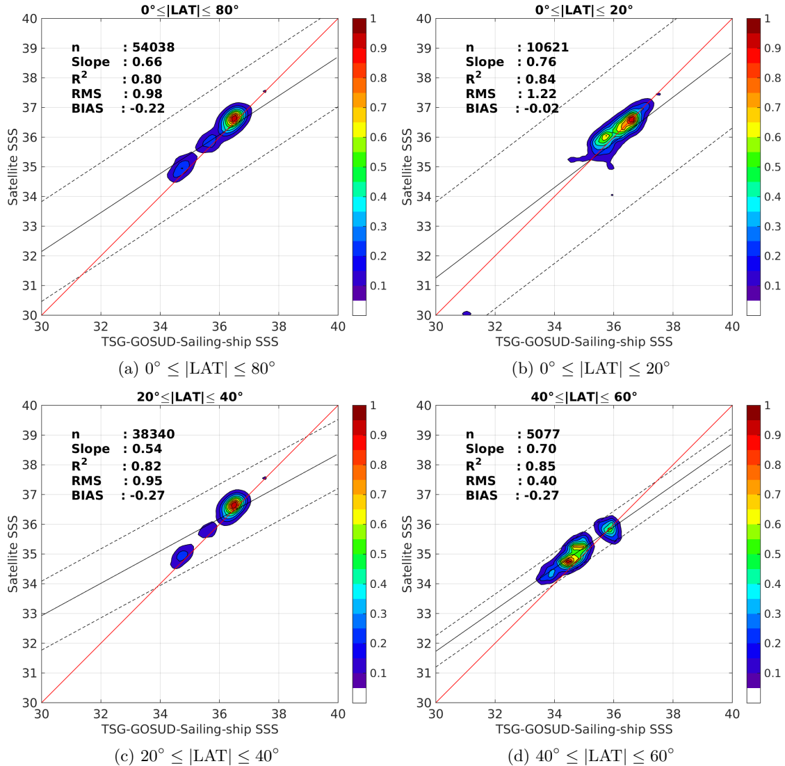
Figure 9: Contour maps of the concentration of Aquarius-L3-JPL-V4-MONTHLY SSS (y-axis) versus TSG-GOSUD-Sailing-ship SSS (x-axis) at match-up pairs for different latitude bands. For each plot, the red line shows x=y . The black thin and dashed lines indicate a linear fit through the data cloud and the \pm 95\% confidence levels, respectively. The number match-up pairs n , the slope and R^2 coefficient of the linear fit, the root mean square (RMS) and the mean bias between satellite and in situ data are indicated for each latitude band in each plots.
