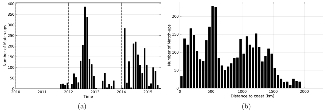
Figure 1: Number of match-ups between Sea mammals and Aquarius-L3-JPL-V4-MONTHLY SSS as a function of time (a) and as function of the distance to coast (b) over the Mid-Low Latitudes 45N-45S Pi-MEP region and for the full satellite product period.
