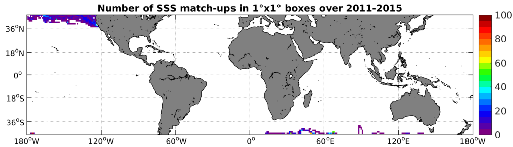
Figure 4: Number of SSS match-ups between Sea mammals SSS and the Aquarius-L3-JPL-V4-MONTHLY SSS product for the Mid-Low Latitudes 45N-45S Pi-MEP region over 1^\circ \times 1^\circ boxes and for the full satellite product period.
