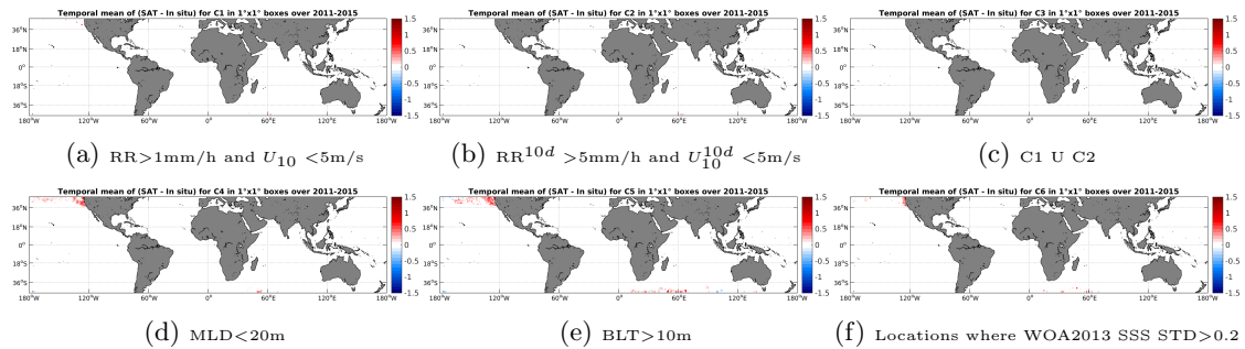
Figure 12: Temporal mean gridded over spatial boxes of size 1^\circ \times 1^\circ of \Delta SSS (Aquarius-L3-JPL-V4-MONTHLY - Sea mammals) for 6 different subdatasets corresponding to: RR>1mm/h and U_{10} < 5\text{m/s} (a), RR^{10d} > 5\text{mm/h} and U_{10}^{10d} < 5\text{m/s} (b), C1 U C2 (c), MLD<20m (d), BLT>10m (e), Locations where WOA2013 SSS STD>0.2 (f).
