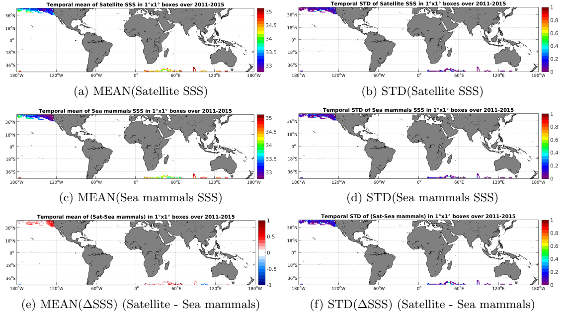
Figure 6: Temporal mean (left) and STD (right) of SSS from Aquarius-L3-JPL-V4-MONTHLY (top), Sea mammals (middle), and of \Delta SSS (Satellite - Sea mammals). Only match-up pairs are used to generate these maps.
