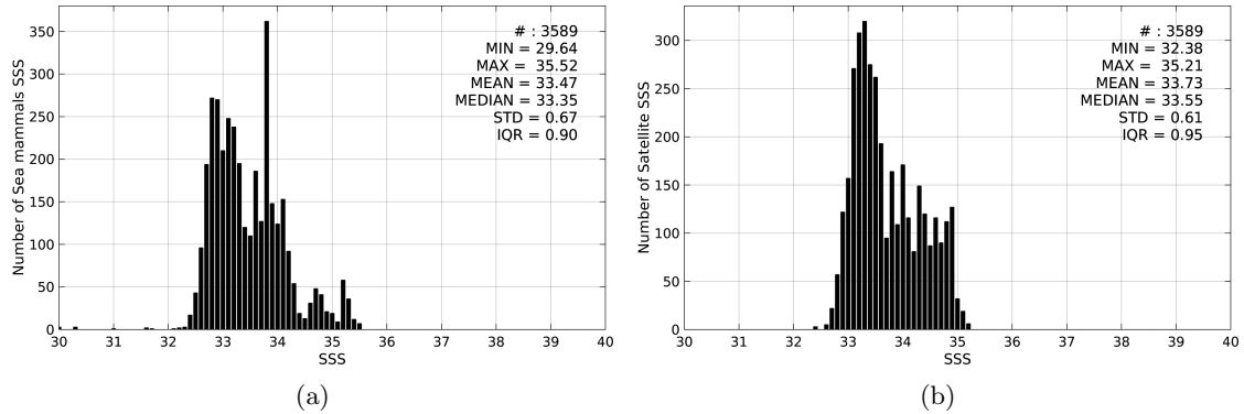
Figure 2: Histograms of SSS from Sea mammals (a) and Aquarius-L3-JPL-V4-MONTHLY (b) considering all match-up pairs per bins of 0.1 over the Mid-Low Latitudes 45N-45S Pi-MEP region and for the full satellite product period.
