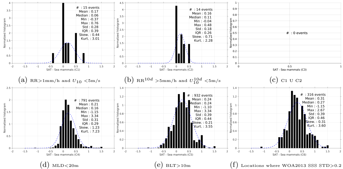
Figure 13: Normalized histogram of \Delta SSS (Aquarius-L3-JPL-V4-MONTHLY - Sea mammals) for 6 different subdatasets corresponding to: RR>1mm/h and U_{10} < 5\text{m/s} (a), RR^{10d} > 5\text{mm/h} and U_{10}^{10d} < 5\text{m/s} (b), C1 U C2 (c), MLD<20m (d), BLT>10m (e), Locations where WOA2013 SSS STD>0.2 (f).
