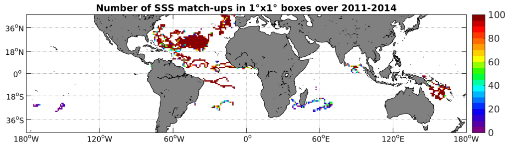
Figure 3: Number of SSS match-ups between Surface drifters SSS and the Aquarius-L3-JPL-V4-MONTHLY SSS product for the Mid-Low Latitudes 45N-45S Pi-MEP region over 1°x1° boxes and for the full satellite product period.
