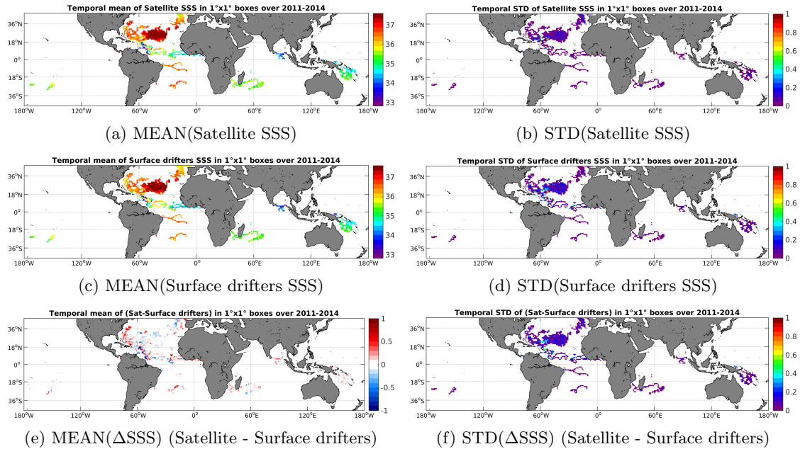
Figure 5: Temporal mean (left) and STD (right) of SSS from Aquarius-L3-JPL-V4-MONTHLY (top), Surface drifters (middle), and of \Delta SSS (Satellite - Surface drifters). Only match-up pairs are used to generate these maps.
