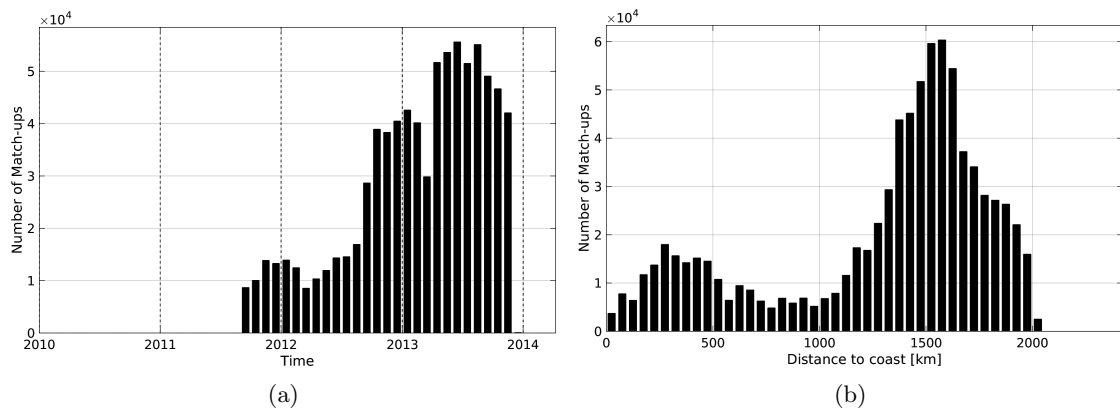
Figure 1: Number of match-ups between Surface drifters and Aquarius-L3-JPL-V4-MONTHLY SSS as a function of time (a) and as function of the distance to coast (b) over the Mid-Low Latitudes 45N-45S Pi-MEP region and for the full satellite product period.
