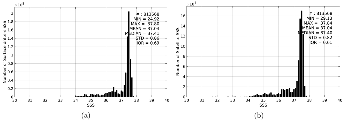
Figure 2: Histograms of SSS from Surface drifters (a) and Aquarius-L3-JPL-V4-MONTHLY (b) considering all match-up pairs per bins of 0.1 over the Mid-Low Latitudes 45N-45S Pi-MEP region and for the full satellite product period.
