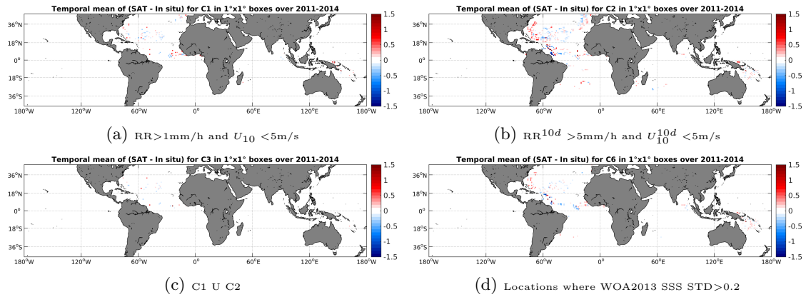
Figure 11: Temporal mean gridded over spatial boxes of size 1^\circ \times 1^\circ of \Delta SSS (Aquarius-L3-JPL-V4-MONTHLY - Surface drifters) for 4 different subdatasets corresponding to: RR > 1\text{mm/h} and U_{10} < 5\text{m/s} (a), RR^{10d} > 5\text{mm/h} and U_{10}^{10d} < 5\text{m/s} (b), C1 U C2 (c), Locations where WOA2013 SSS STD > 0.2 (d).
