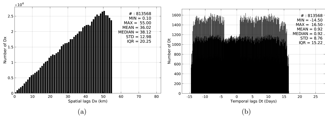
Figure 4: Histograms of the spatial (a) and temporal (b) lags between the time of the Surface drifters measurements and the date of the corresponding Aquarius-L3-JPL-V4-MONTHLY SSS product.
