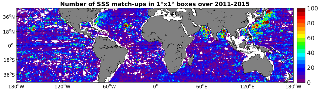
Figure 4: Number of SSS match-ups between Argo SSS and the Aquarius-L3-JPL-V4-MONTHLY SSS product for the Mid-Low Latitudes 45N-45S Pi-MEP region over 1^\circ \times 1^\circ boxes and for the full satellite product period.
