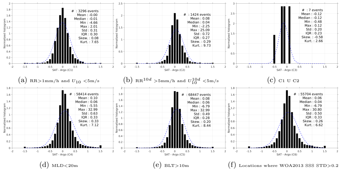
Figure 13: Normalized histogram of \Delta SSS (Aquarius-L3-JPL-V4-MONTHLY - Argo) for 6 different subdatasets corresponding to: RR > 1 mm/h and U_{10} < 5 m/s (a), RR ^{10d} > 5 mm/h and U_{10}^{10d} < 5 m/s (b), C1 U C2 (c), MLD < 20 m (d), BLT > 10 m (e), Locations where WOA2013 SSS STD > 0.2 (f).
