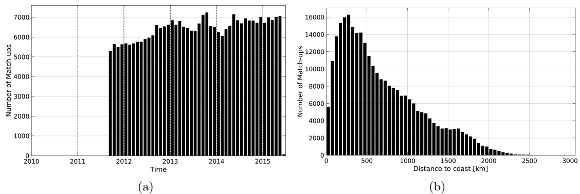
Figure 1: Number of match-ups between Argo and Aquarius-L3-JPL-V4-MONTHLY SSS as a function of time (a) and as function of the distance to coast (b) over the Mid-Low Latitudes 45N-45S Pi-MEP region and for the full satellite product period.
