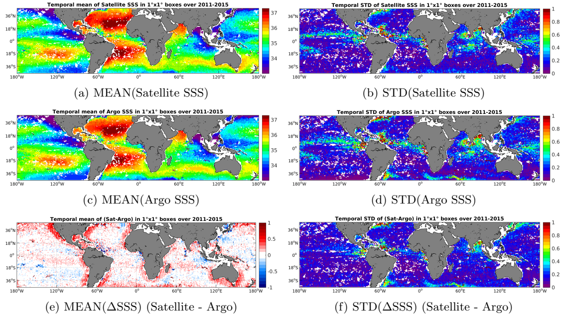
Figure 6: Temporal mean (left) and STD (right) of SSS from Aquarius-L3-JPL-V4-MONTHLY (top), Argo (middle), and of \Delta SSS (Satellite - Argo). Only match-up pairs are used to generate these maps.
