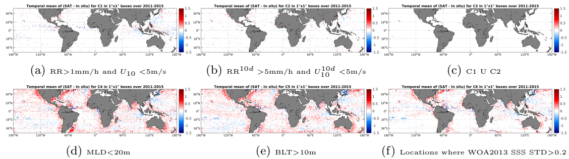
Figure 12: Temporal mean gridded over spatial boxes of size 1^\circ \times 1^\circ of \Delta SSS (Aquarius-L3-JPL-V4-MONTHLY - Argo) for 6 different subdatasets corresponding to: RR > 1 mm/h and U_{10} < 5 m/s (a), RR ^{10d} > 5 mm/h and U_{10}^{10d} < 5 m/s (b), C1 U C2 (c), MLD < 20 m (d), BLT > 10 m (e), Locations where WOA2013 SSS STD > 0.2 (f).
