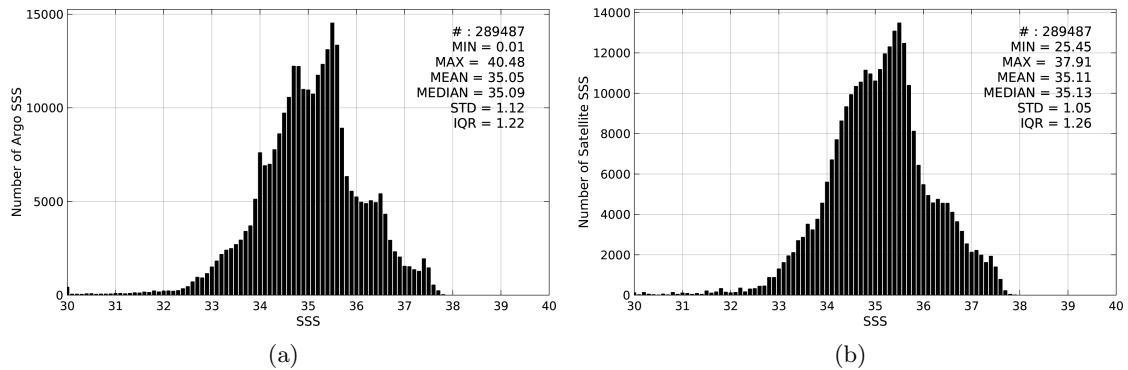
Figure 2: Histograms of SSS from Argo (a) and Aquarius-L3-JPL-V4-MONTHLY (b) considering all match-up pairs per bins of 0.1 over the Mid-Low Latitudes 45N-45S Pi-MEP region and for the full satellite product period.
