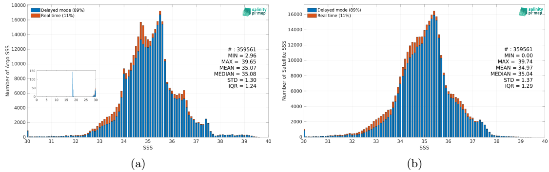
Figure 2: Histograms of SSS from Argo (a) and Aquarius SSS L2-AVERAGED OR v5 (NASA-GSFC) (b) considering all match-up pairs per bins of 0.1 over the Mid-Low Latitudes 45N-45S Pi-MEP region and for the full satellite product period.
