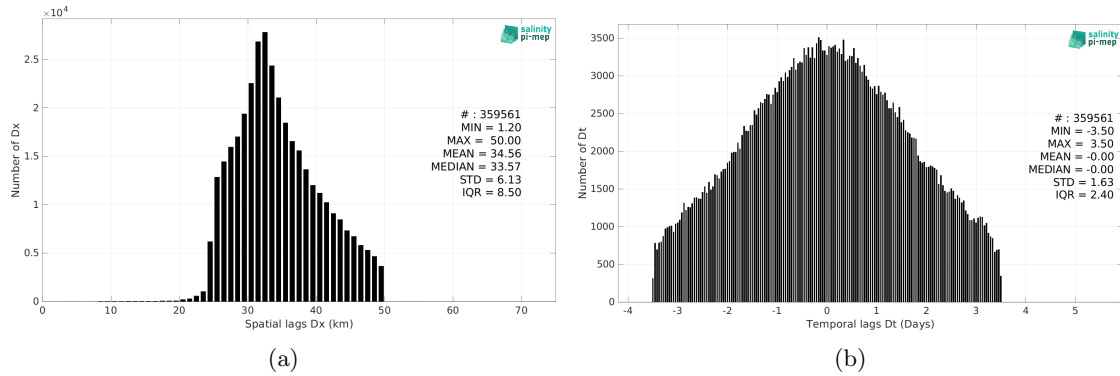
Figure 5: Histograms of the spatial (a) and temporal (b) lags between the location/time of the Argo measurement and the date of the corresponding Aquarius SSS L2-AVERAGED OR v5 (NASA-GSFC) SSS pixel.
