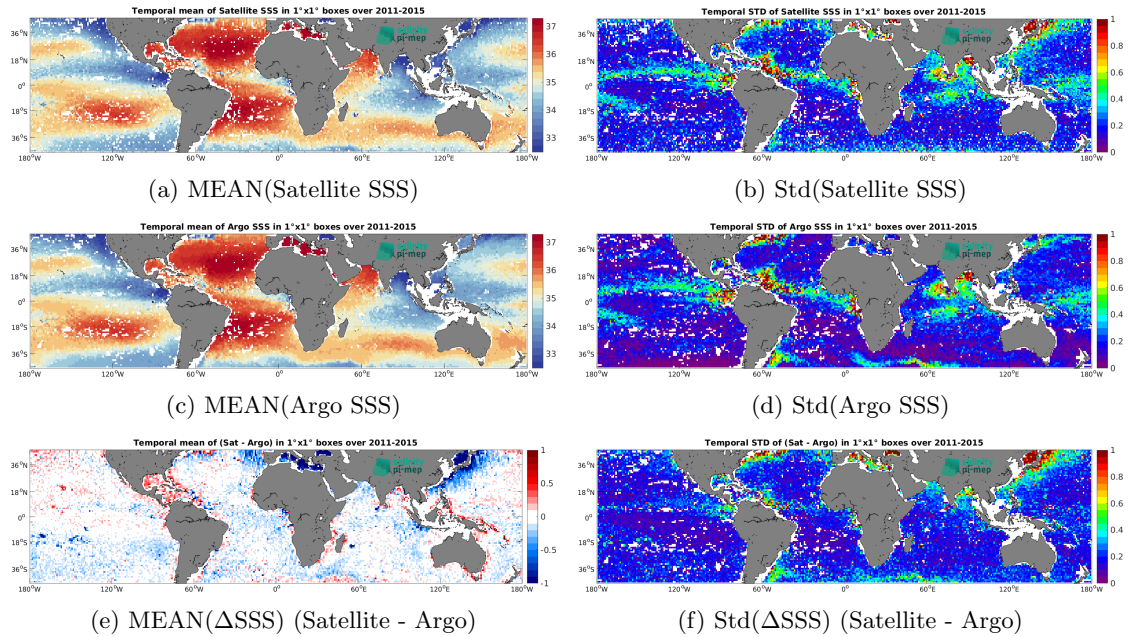
Figure 6: Temporal mean (left) and Std (right) of SSS from Aquarius SSS L2-AVERAGED OR v5 (NASA-GSFC) (top), Argo (middle), and of \Delta SSS (Satellite - Argo). Only match-up pairs are used to generate these maps.
