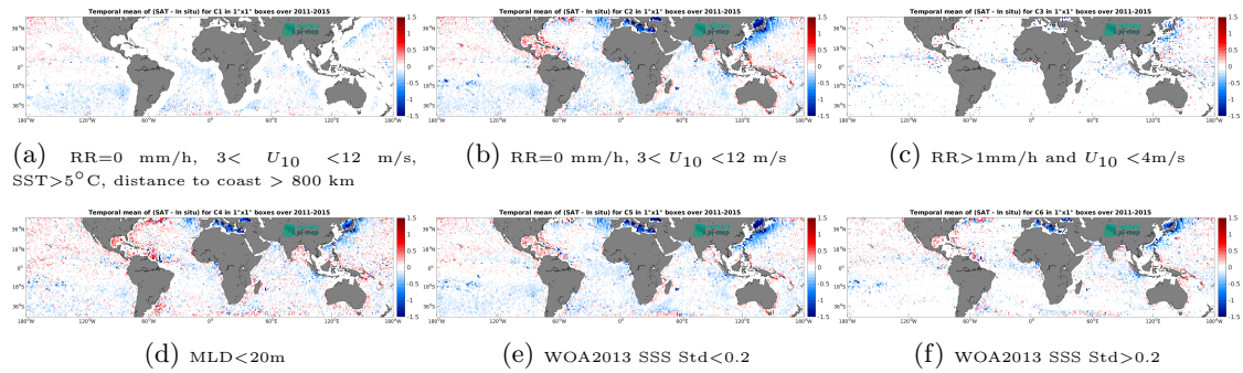
Figure 12: Temporal mean gridded over spatial boxes of size 1^\circ \times 1^\circ of \Delta SSS (Aquarius SSS L2-AVERAGED OR v5 (NASA-GSFC) - Argo) for 6 different subdatasets corresponding to:RR=0 mm/h, 3 < U_{10} < 12 m/s, SST >5^\circ C, distance to coast > 800 km (a), RR=0 mm/h, 3 < U_{10} < 12 m/s (b), RR >1 mm/h and U_{10} < 4 m/s (c),MLD <20 m (d),WOA2013 SSS Std <0.2 (e),WOA2013 SSS Std >0.2 (f).
