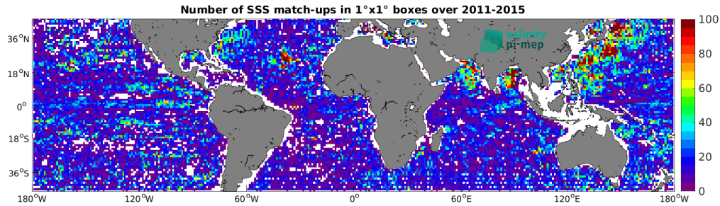
Figure 4: Number of SSS match-ups between Argo SSS and the Aquarius SSS L2-AVERAGED OR v5 (NASA-GSFC) SSS product for the Mid-Low Latitudes 45N-45S Pi-MEP region over 1^\circ \times 1^\circ boxes and for the full satellite product period.
