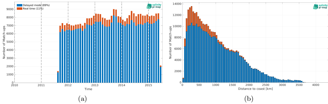
Figure 1: Number of match-ups between Argo and Aquarius SSS L2-AVERAGED OR v5 (NASA-GSFC) SSS as a function of time (a) and as function of the distance to coast (b) over the Mid-Low Latitudes 45N-45S Pi-MEP region and for the full satellite product period.
