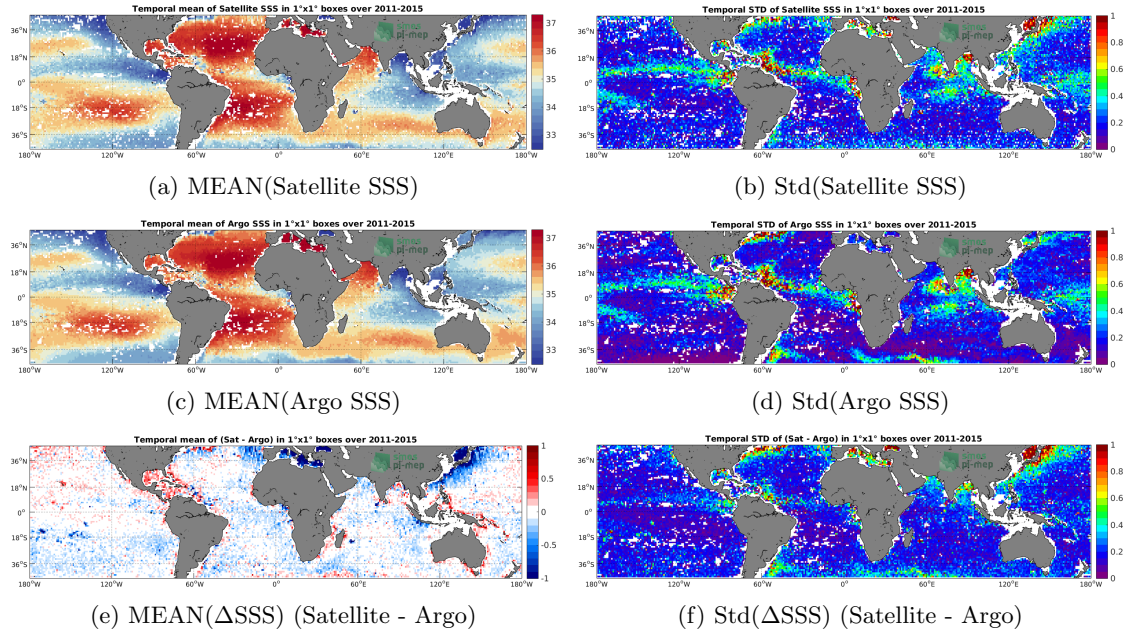
Figure 6: Temporal mean (left) and Std (right) of SSS from Aquarius SSS L2-AVERAGED OR v5 (NASA-GSFC) (top), Argo (middle), and of \Delta SSS (Satellite - Argo). Only match-up pairs are used to generate these maps.
