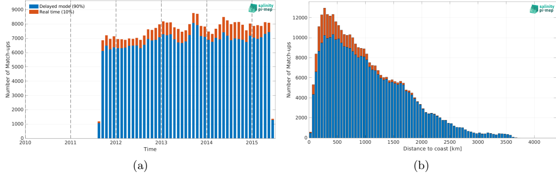
Figure 1: Number of match-ups between Argo and Aquarius SSS L2-AVERAGED CAP v5 (JPL) SSS as a function of time (a) and as function of the distance to coast (b) over the Mid-Low Latitudes 45N-45S Pi-MEP region and for the full satellite product period.
