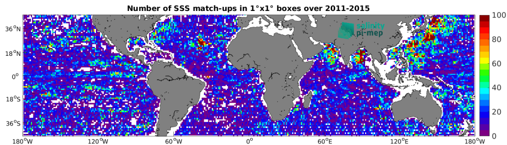
Figure 4: Number of SSS match-ups between Argo SSS and the Aquarius SSS L2-AVERAGED CAP v5 (JPL) SSS product for the Mid-Low Latitudes 45N-45S Pi-MEP region over 1^\circ \times 1^\circ boxes and for the full satellite product period.
