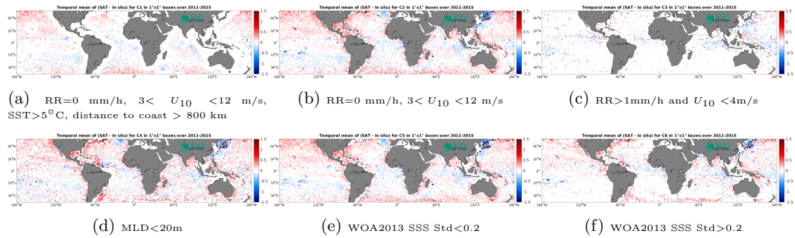
Figure 12: Temporal mean gridded over spatial boxes of size 1^\circ \times 1^\circ of \Delta SSS (Aquarius SSS L2-AVERAGED CAP v5 (JPL) - Argo) for 6 different subdatasets corresponding to:RR=0 mm/h, 3 < U_{10} < 12 m/s, SST >5^\circ C, distance to coast > 800 km (a), RR=0 mm/h, 3 < U_{10} < 12 m/s (b), RR >1 mm/h and U_{10} < 4 m/s (c),MLD <20 m (d),WOA2013 SSS Std <0.2 (e),WOA2013 SSS Std >0.2 (f).
