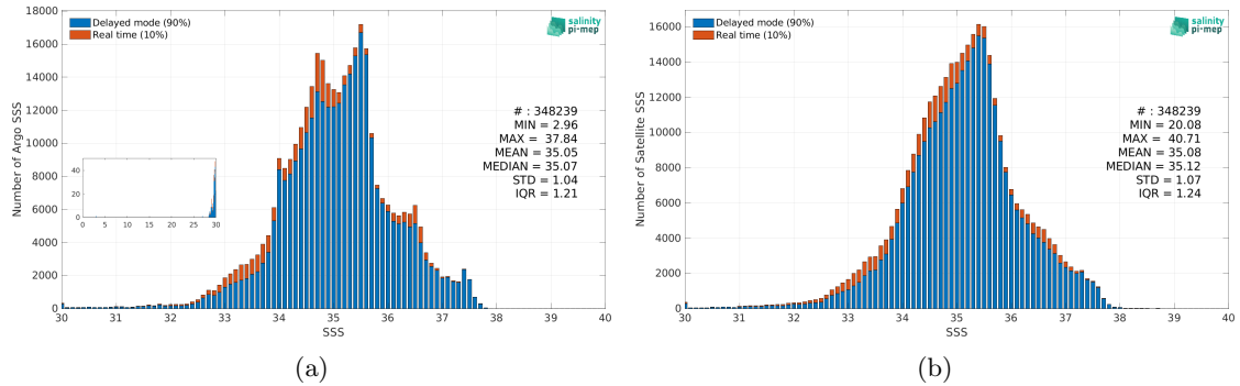
Figure 2: Histograms of SSS from Argo (a) and Aquarius SSS L2-AVERAGED CAP v5 (JPL) (b) considering all match-up pairs per bins of 0.1 over the Mid-Low Latitudes 45N-45S Pi-MEP region and for the full satellite product period.
