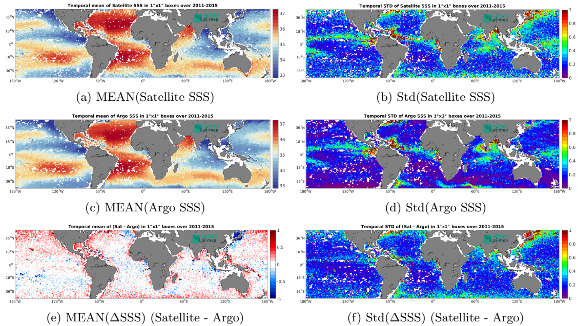
Figure 6: Temporal mean (left) and Std (right) of SSS from Aquarius SSS L2-AVERAGED CAP v5 (JPL) (top), Argo (middle), and of \Delta SSS (Satellite - Argo). Only match-up pairs are used to generate these maps.
