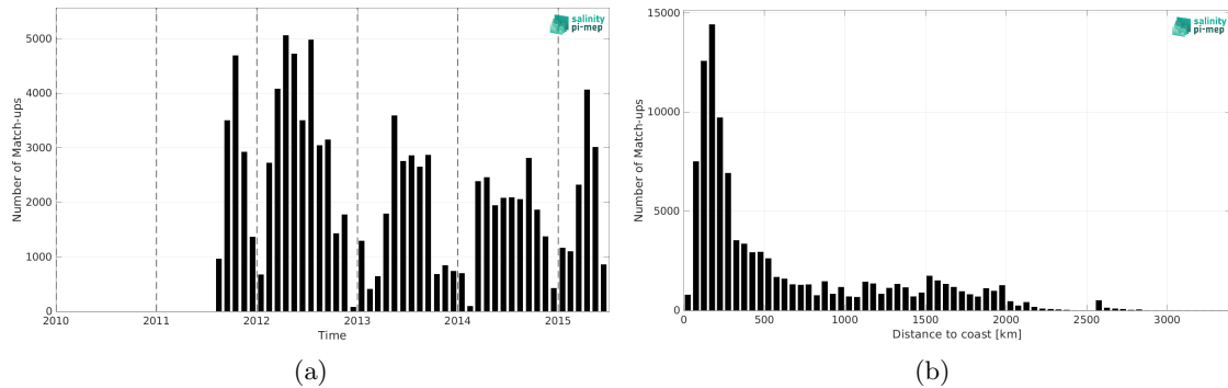
Figure 2: Number of match-ups between TSG (SAMOS) and Aquarius SSS L2 OR v5 (NASA-GSFC) SSS as a function of time (a) and as function of the distance to coast (b) over the Mid-Low Latitudes 45N-45S Pi-MEP region and for the full satellite product period.
