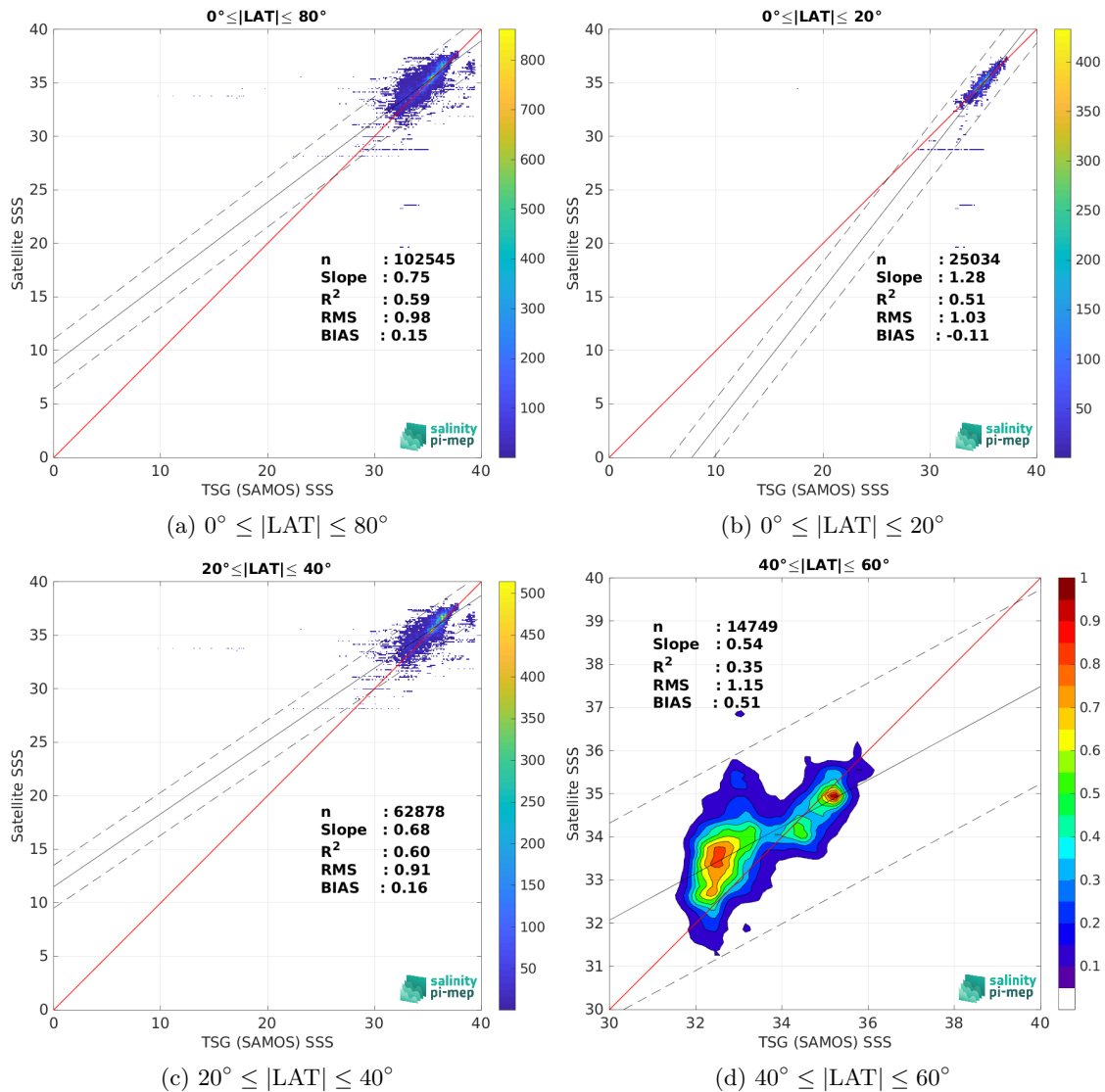
Figure 10: Contour maps of the concentration of Aquarius SSS L2 OR v5 (NASA-GSFC) SSS (y-axis) versus TSG (SAMOS) SSS (x-axis) at match-up pairs for different latitude bands. For each plot, the red line shows x=y . The black thin and dashed lines indicate a linear fit through the data cloud and the \pm 95\% confidence levels, respectively. The number match-up pairs n , the slope and R^2 coefficient of the linear fit, the root mean square (RMS) and the mean bias between satellite and in situ data are indicated for each latitude band in each plots.
