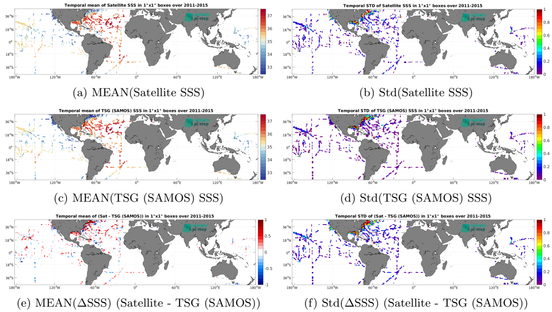
Figure 7: Temporal mean (left) and Std (right) of SSS from Aquarius SSS L2 OR v5 (NASA-GSFC) (top), TSG (SAMOS) ( in situ ) (middle), and of \Delta SSS (Satellite - TSG (SAMOS)). Only match-up pairs are used to generate these maps.
