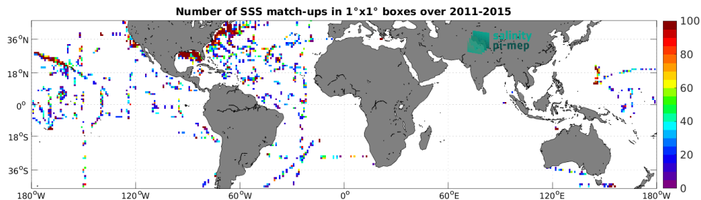
Figure 5: Number of SSS match-ups between TSG (SAMOS) SSS and the Aquarius SSS L2 OR v5 (NASA-GSFC) SSS product for the Mid-Low Latitudes 45N-45S Pi-MEP region over 1^\circ \times 1^\circ boxes and for the full satellite product period.
