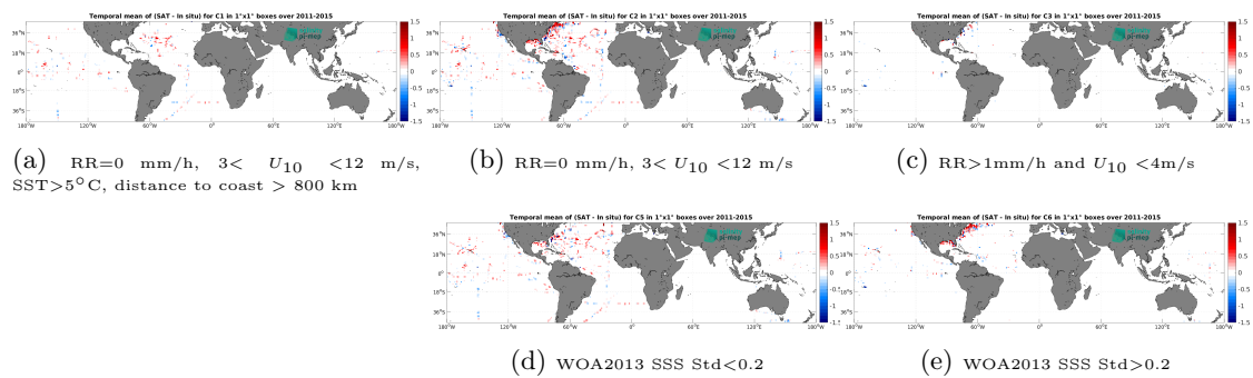
Figure 14: Temporal mean gridded over spatial boxes of size 1^\circ \times 1^\circ of \Delta SSS (Aquarius SSS L2 OR v5 (NASA-GSFC) - TSG (SAMOS)) for 5 different subdatasets corresponding to: RR=0 mm/h, 3 < U_{10} < 12 m/s, SST > 5^\circ\text{C} , distance to coast > 800 km (a), RR=0 mm/h, 3 < U_{10} < 12 m/s (b), RR > 1\text{mm/h} and U_{10} < 4\text{m/s} (c), WOA2013 SSS Std < 0.2 (d), WOA2013 SSS Std > 0.2 (e).
