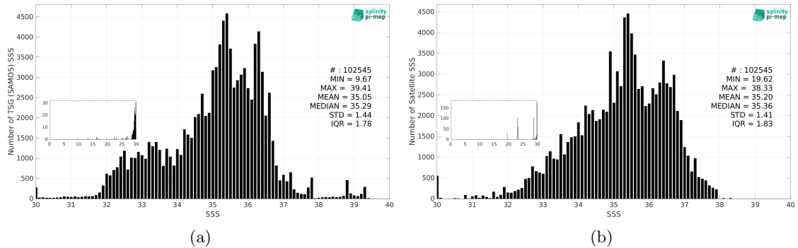
Figure 3: Histograms of SSS from TSG (SAMOS) (a) and Aquarius SSS L2 OR v5 (NASA-GSFC) (b) considering all match-up pairs per bins of 0.1 over the Mid-Low Latitudes 45N-45S Pi-MEP region and for the full satellite product period.
