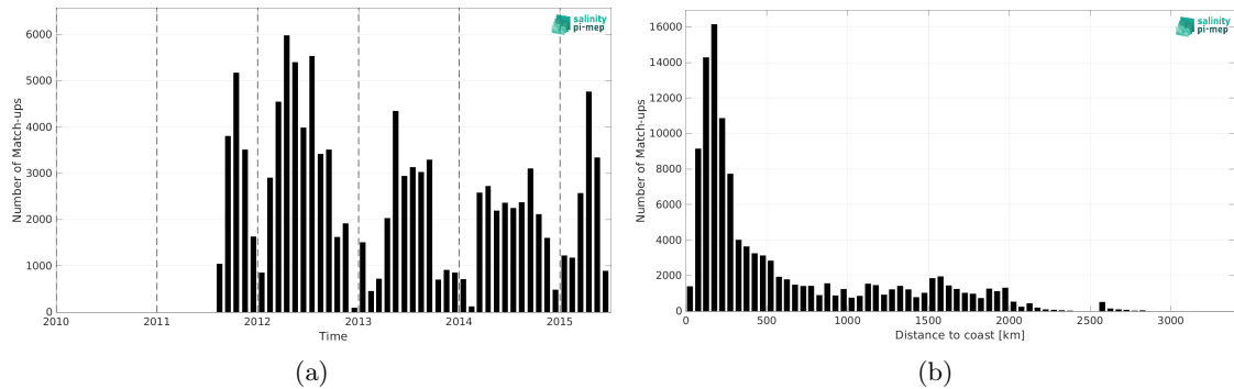
Figure 1: Number of match-ups between TSG (SAMOS) and Aquarius SSS L2 OR v5 (NASA-GSFC) SSS as a function of time (a) and as function of the distance to coast (b) over the Mid-Low Latitudes 45N-45S Pi-MEP region and for the full satellite product period.
