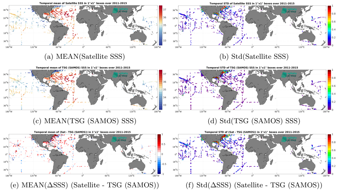
Figure 6: Temporal mean (left) and Std (right) of SSS from Aquarius SSS L2 OR v5 (NASA-GSFC) (top), TSG (SAMOS) (middle), and of \Delta SSS (Satellite - TSG (SAMOS)). Only match-up pairs are used to generate these maps.
