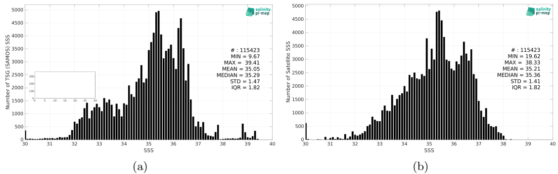
Figure 2: Histograms of SSS from TSG (SAMOS) (a) and Aquarius SSS L2 OR v5 (NASA-GSFC) (b) considering all match-up pairs per bins of 0.1 over the Mid-Low Latitudes 45N-45S Pi-MEP region and for the full satellite product period.
