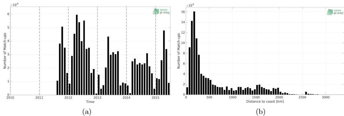
Figure 1: Number of match-ups between TSG (SAMOS) and Aquarius SSS L2 OR v5 (NASA-GSFC) SSS as a function of time (a) and as function of the distance to coast (b) over the Mid-Low Latitudes 45N-45S Pi-MEP region and for the full satellite product period.
