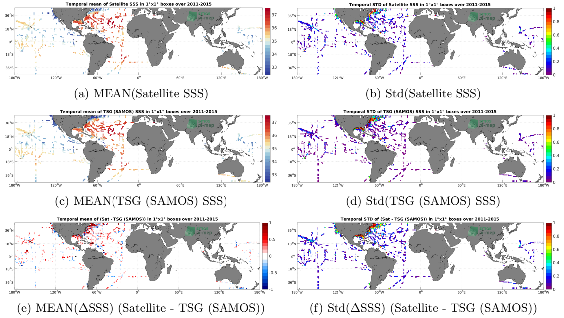
Figure 6: Temporal mean (left) and Std (right) of SSS from Aquarius SSS L2 OR v5 (NASA-GSFC) (top), TSG (SAMOS) ( in situ ) dataset (middle), and of \Delta SSS (Satellite - TSG (SAMOS)). Only match-up pairs are used to generate these maps.
