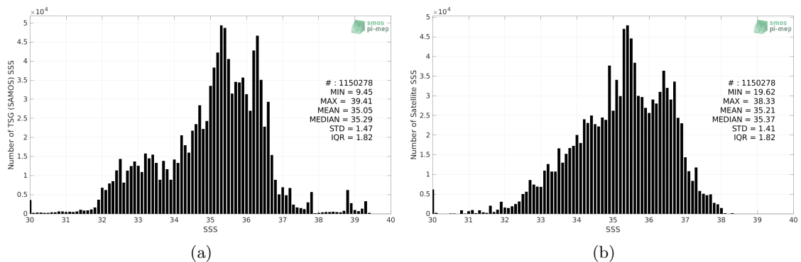
Figure 2: Histograms of SSS from TSG (SAMOS) (a) and Aquarius SSS L2 OR v5 (NASA-GSFC) (b) considering all match-up pairs per bins of 0.1 over the Mid-Low Latitudes 45N-45S Pi-MEP region and for the full satellite product period.
