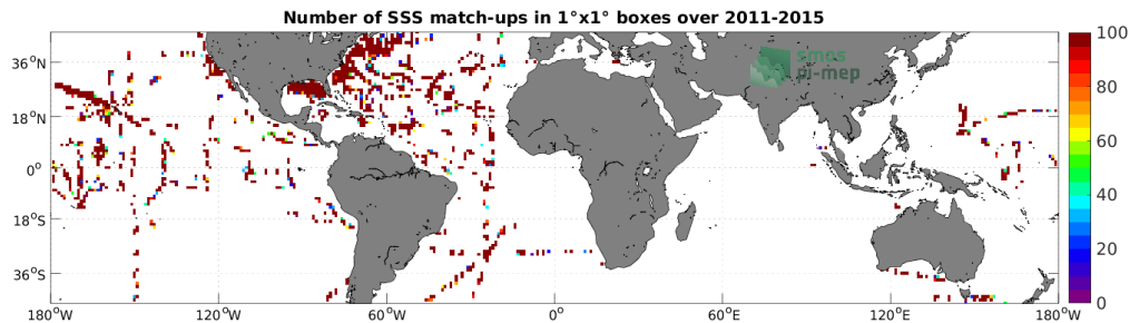
Figure 4: Number of SSS match-ups between TSG (SAMOS) SSS and the Aquarius SSS L2 OR v5 (NASA-GSFC) SSS product for the Mid-Low Latitudes 45N-45S Pi-MEP region over 1^\circ \times 1^\circ boxes and for the full satellite product period.
