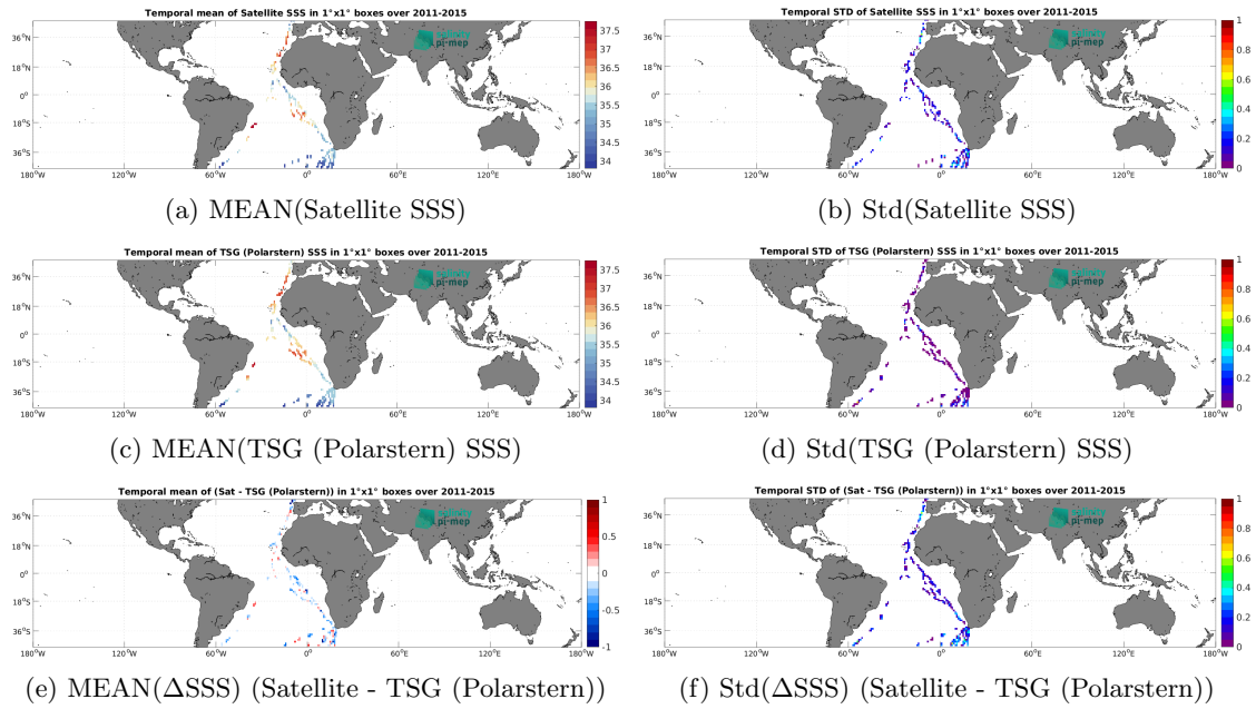
Figure 7: Temporal mean (left) and Std (right) of SSS from Aquarius SSS L2 OR v5 (NASA-GSFC) (top), TSG (Polarstern) (middle), and of \Delta SSS (Satellite - TSG (Polarstern)). Only match-up pairs are used to generate these maps.
