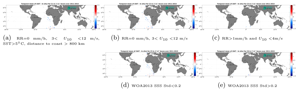
Figure 14: Temporal mean gridded over spatial boxes of size 1^\circ \times 1^\circ of \Delta SSS (Aquarius SSS L2 OR v5 (NASA-GSFC) - TSG (Polarstern)) for 5 different subdatasets corresponding to: RR=0 mm/h, 3 < U_{10} < 12 m/s, SST > 5^\circ\text{C} , distance to coast > 800 km (a), RR=0 mm/h, 3 < U_{10} < 12 m/s (b), RR > 1 mm/h and U_{10} < 4 m/s (c), WOA2013 SSS Std < 0.2 (d), WOA2013 SSS Std > 0.2 (e).
