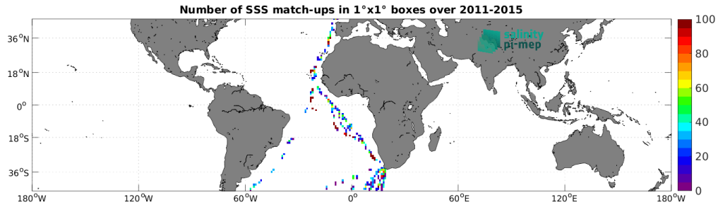
Figure 5: Number of SSS match-ups between TSG (Polarstern) SSS and the Aquarius SSS L2 OR v5 (NASA-GSFC) SSS product for the Mid-Low Latitudes 45N-45S Pi-MEP region over 1^\circ \times 1^\circ boxes and for the full satellite product period.
