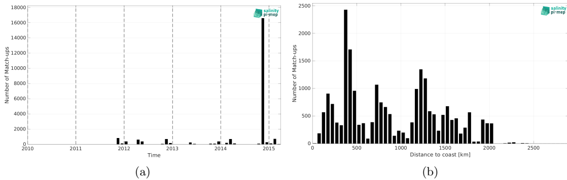
Figure 2: Number of match-ups between TSG (Polarstern) and Aquarius SSS L2 OR v5 (NASA-GSFC) SSS as a function of time (a) and as function of the distance to coast (b) over the Mid-Low Latitudes 45N-45S Pi-MEP region and for the full satellite product period.
