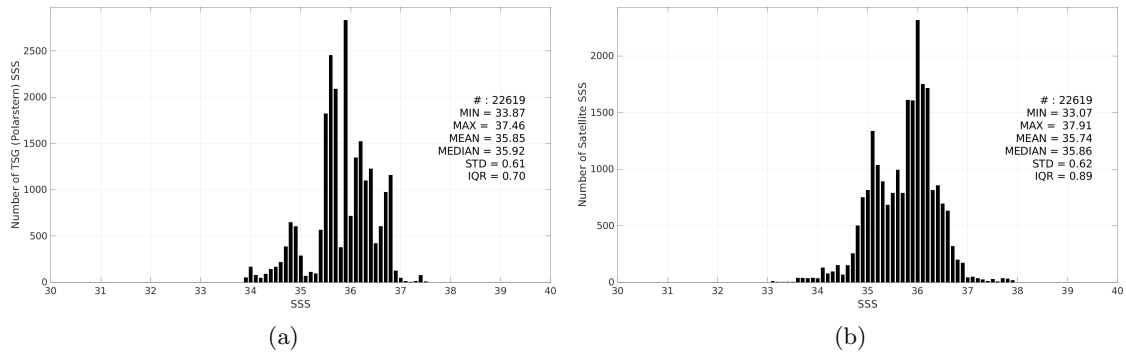
Figure 3: Histograms of SSS from TSG (Polarstern) (a) and Aquarius SSS L2 OR v5 (NASA-GSFC) (b) considering all match-up pairs per bins of 0.1 over the Mid-Low Latitudes 45N-45S Pi-MEP region and for the full satellite product period.
