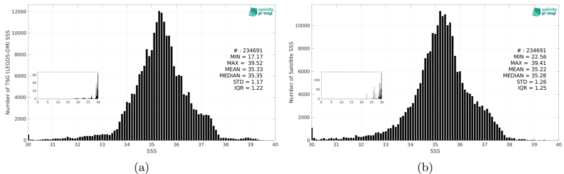
Figure 3: Histograms of SSS from TSG (LEGOS-DM) (a) and Aquarius SSS L2 OR v5 (NASA-GSFC) (b) considering all match-up pairs per bins of 0.1 over the Mid-Low Latitudes 45N-45S Pi-MEP region and for the full satellite product period.
