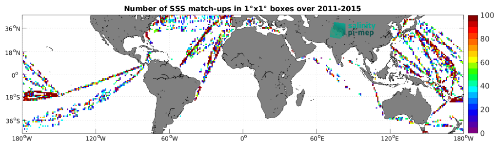
Figure 5: Number of SSS match-ups between TSG (LEGOS-DM) SSS and the Aquarius SSS L2 OR v5 (NASA-GSFC) SSS product for the Mid-Low Latitudes 45N-45S Pi-MEP region over 1^\circ \times 1^\circ boxes and for the full satellite product period.
