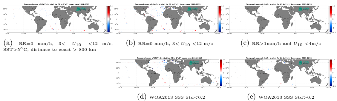
Figure 14: Temporal mean gridded over spatial boxes of size 1^\circ \times 1^\circ of \Delta\text{SSS} (Aquarius SSS L2 OR v5 (NASA-GSFC) - TSG (GOSUD-Sailing-ship)) for 5 different subdatasets corresponding to:RR=0 mm/h, 3 < U_{10} < 12 m/s, SST>5°C, distance to coast > 800 km (a), RR=0 mm/h, 3 < U_{10} < 12 m/s (b), RR>1mm/h and U_{10} < 4 m/s (c), WOA2013 SSS Std<0.2 (d), WOA2013 SSS Std>0.2 (e).
