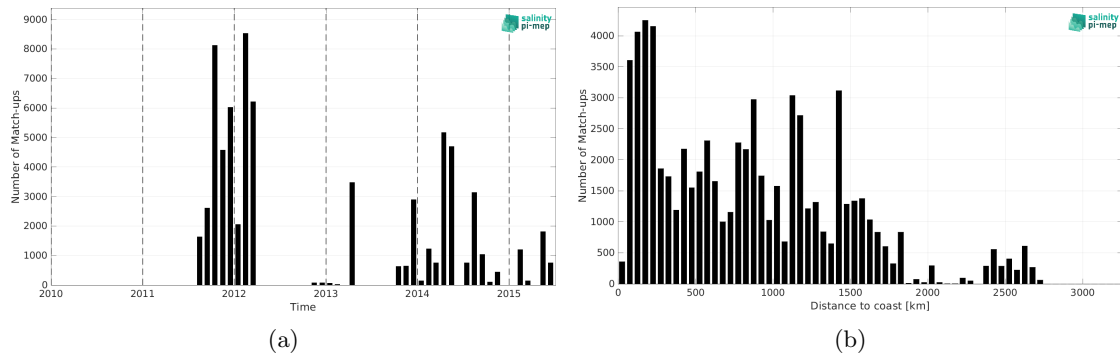
Figure 2: Number of match-ups between TSG (GOSUD-Sailing-ship) and Aquarius SSS L2 OR v5 (NASA-GSFC) SSS as a function of time (a) and as function of the distance to coast (b) over the Mid-Low Latitudes 45N-45S Pi-MEP region and for the full satellite product period.
