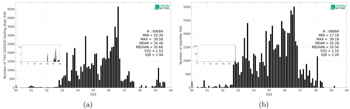
Figure 3: Histograms of SSS from TSG (GOSUD-Sailing-ship) (a) and Aquarius SSS L2 OR v5 (NASA-GSFC) (b) considering all match-up pairs per bins of 0.1 over the Mid-Low Latitudes 45N-45S Pi-MEP region and for the full satellite product period.
