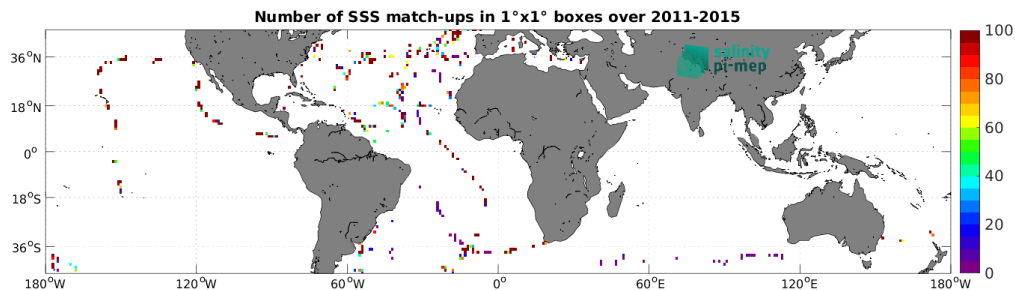
Figure 5: Number of SSS match-ups between TSG (GOSUD-Sailing-ship) SSS and the Aquarius SSS L2 OR v5 (NASA-GSFC) SSS product for the Mid-Low Latitudes 45N-45S Pi-MEP region over 1^\circ \times 1^\circ boxes and for the full satellite product period.
