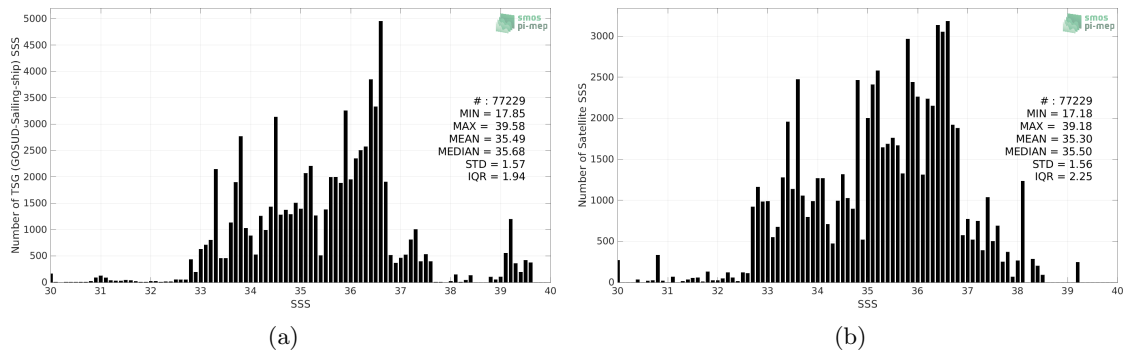
Figure 2: Histograms of SSS from TSG (GOSUD-Sailing-ship) (a) and Aquarius SSS L2 OR v5 (NASA-GSFC) (b) considering all match-up pairs per bins of 0.1 over the Mid-Low Latitudes 45N-45S Pi-MEP region and for the full satellite product period.
