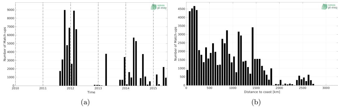
Figure 1: Number of match-ups between TSG (GOSUD-Sailing-ship) and Aquarius SSS L2 OR v5 (NASA-GSFC) SSS as a function of time (a) and as function of the distance to coast (b) over the Mid-Low Latitudes 45N-45S Pi-MEP region and for the full satellite product period.
