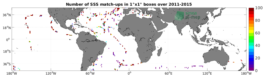
Figure 4: Number of SSS match-ups between TSG (GOSUD-Sailing-ship) SSS and the Aquarius SSS L2 OR v5 (NASA-GSFC) SSS product for the Mid-Low Latitudes 45N-45S Pi-MEP region over 1^\circ \times 1^\circ boxes and for the full satellite product period.
