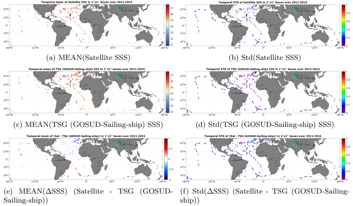
Figure 6: Temporal mean (left) and Std (right) of SSS from Aquarius SSS L2 OR v5 (NASA-GSFC) (top), TSG (GOSUD-Sailing-ship) (middle), and of \Delta SSS (Satellite - TSG (GOSUD-Sailing-ship)). Only match-up pairs are used to generate these maps.
