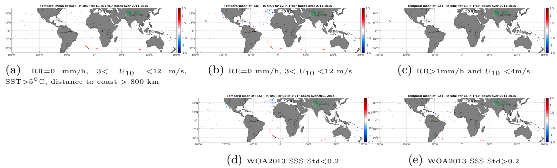
Figure 12: Temporal mean gridded over spatial boxes of size 1^\circ \times 1^\circ of \Delta\text{SSS} (Aquarius SSS L2 OR v5 (NASA-GSFC) - TSG (GOSUD-Sailing-ship)) for 5 different subdatasets corresponding to: RR=0 mm/h, 3 < U_{10} < 12 m/s, SST > 5°C, distance to coast > 800 km (a), RR=0 mm/h, 3 < U_{10} < 12 m/s (b), RR > 1mm/h and U_{10} < 4 m/s (c), WOA2013 SSS Std < 0.2 (d), WOA2013 SSS Std > 0.2 (e).
